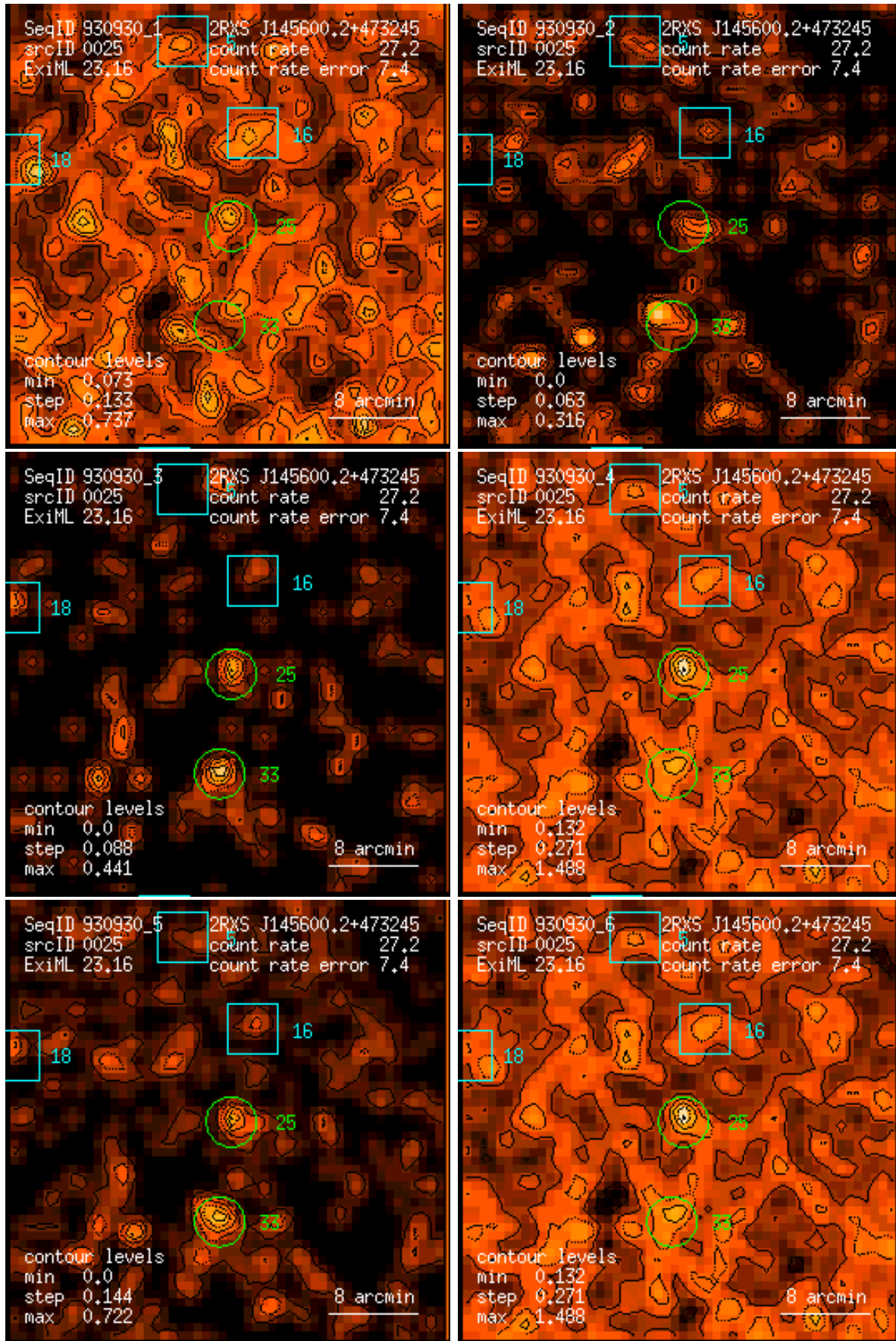
Figure 25: RASS 930930: detection 0025: band rate images, Gaussian filter: (1) PSPC channels 11 – 41, (2) 52 – 90, (3) 91 – 201, (4) 11 – 235, (5) 52 – 201, (6) 11 – 201. Broad band rates in counts/ks. Band rate contour levels in counts/ks/arcmin 2 .
