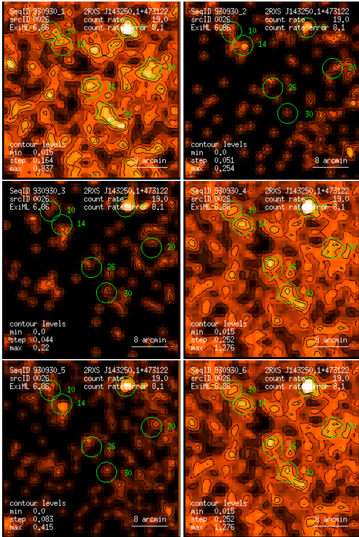
Figure 26: RASS 930930: detection 0026: band rate images, Gaussian filter: (1) PSPC channels 11 – 41, (2) 52 – 90, (3) 91 – 201, (4) 11 – 235, (5) 52 – 201, (6) 11 – 201. Broad band rates in counts/ks. Band rate contour levels in counts/ks/arcmin 2 .
