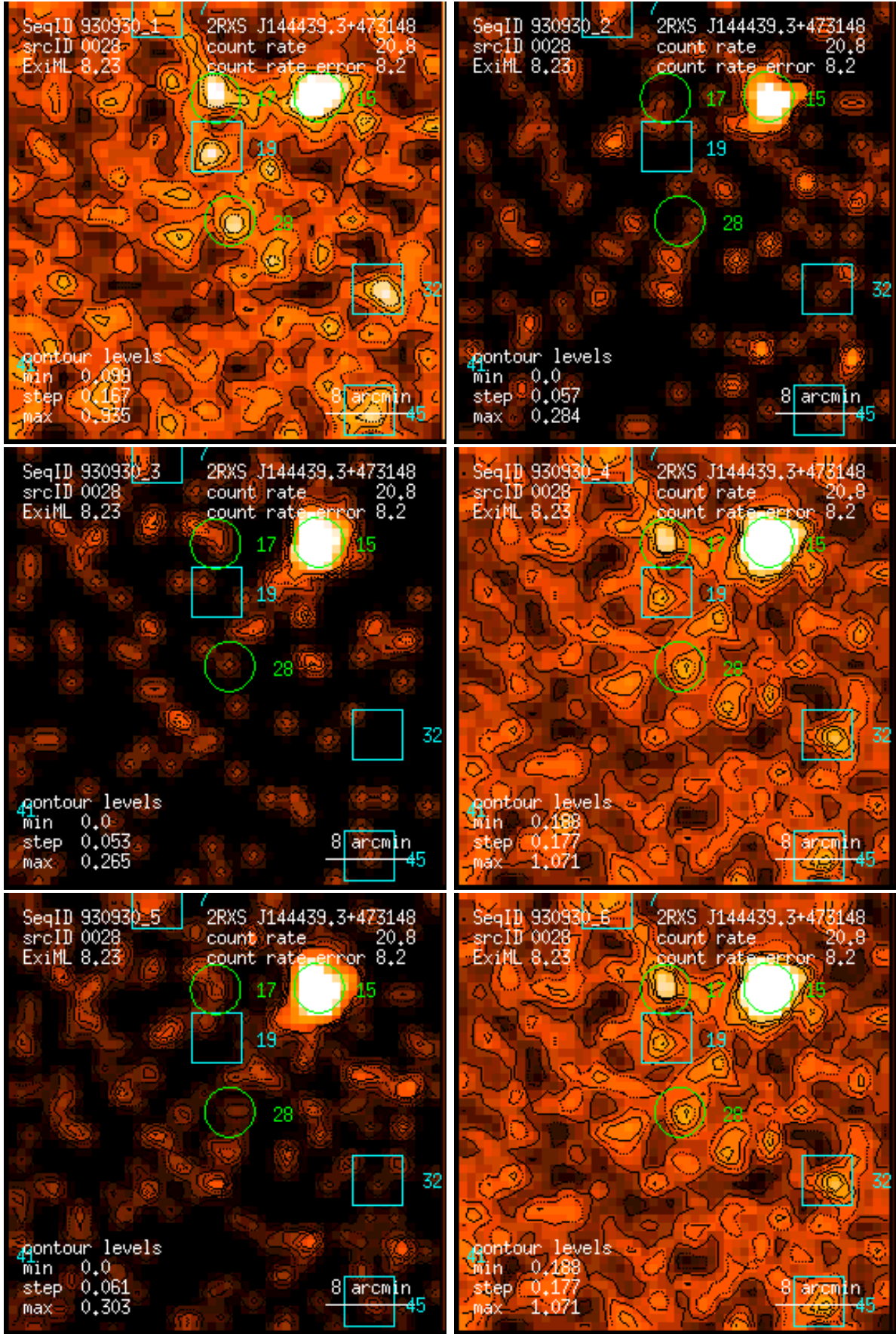
Figure 28: RASS 930930: detection 0028: band rate images, Gaussian filter: (1) PSPC channels 11 – 41, (2) 52 – 90, (3) 91 – 201, (4) 11 – 235, (5) 52 – 201, (6) 11 – 201. Broad band rates in counts/ks. Band rate contour levels in counts/ks/arcmin 2 .
