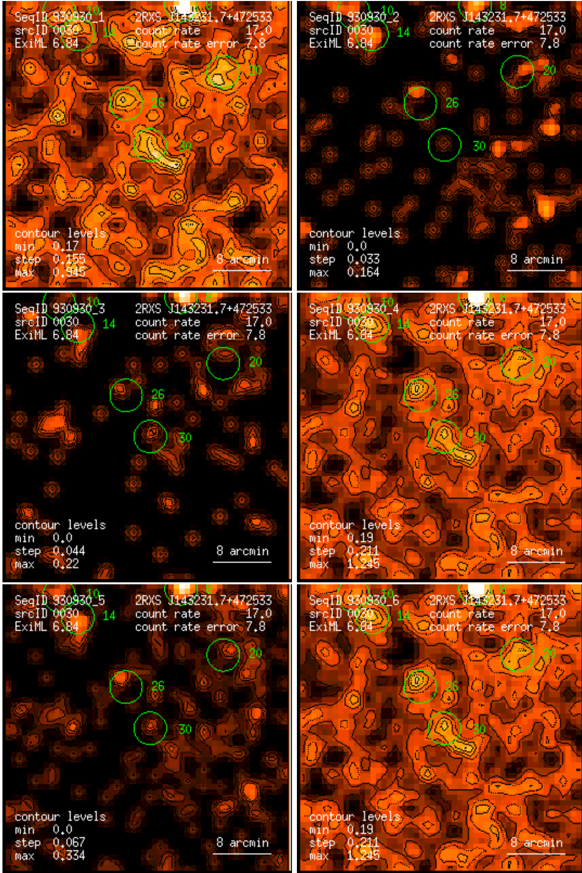
Figure 30: RASS 930930: detection 0030: band rate images, Gaussian filter: (1) PSPC channels 11 – 41, (2) 52 – 90, (3) 91 – 201, (4) 11 – 235, (5) 52 – 201, (6) 11 – 201. Broad band rates in counts/ks. Band rate contour levels in counts/ks/arcmin 2 .
