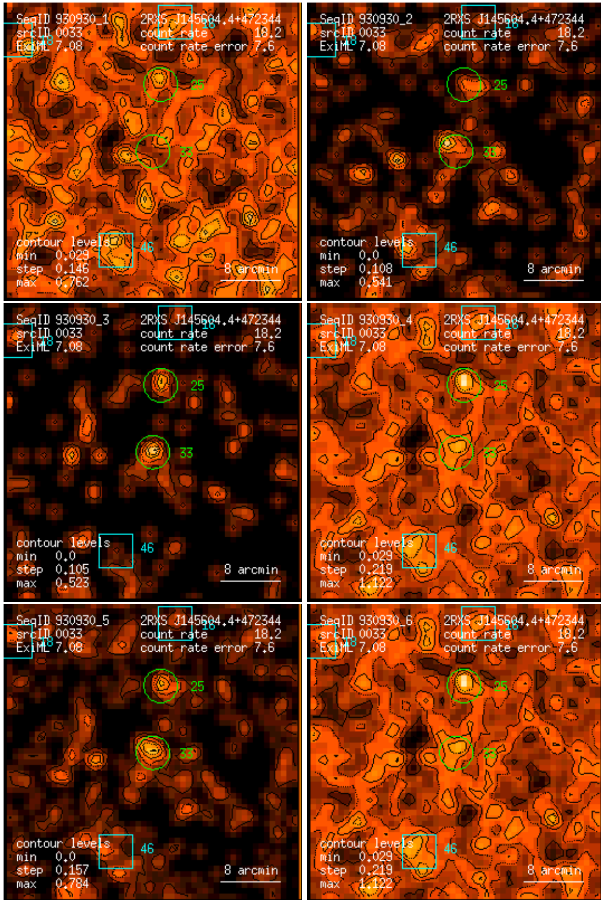
Figure 33: RASS 930930: detection 0033: band rate images, Gaussian filter: (1) PSPC channels 11 – 41, (2) 52 – 90, (3) 91 – 201, (4) 11 – 235, (5) 52 – 201, (6) 11 – 201. Broad band rates in counts/ks. Band rate contour levels in counts/ks/arcmin 2 .
