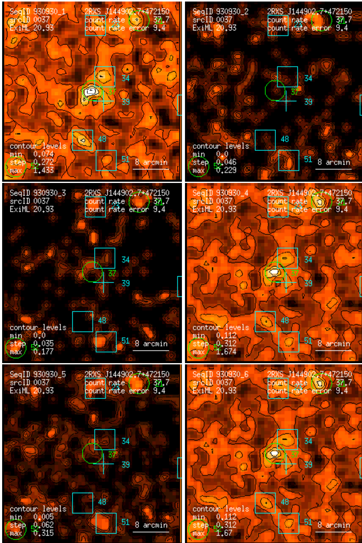
Figure 37: RASS 930930: detection 0037: band rate images, Gaussian filter: (1) PSPC channels 11 – 41, (2) 52 – 90, (3) 91 – 201, (4) 11 – 235, (5) 52 – 201, (6) 11 – 201. Broad band rates in counts/ks. Band rate contour levels in counts/ks/arcmin 2 .
