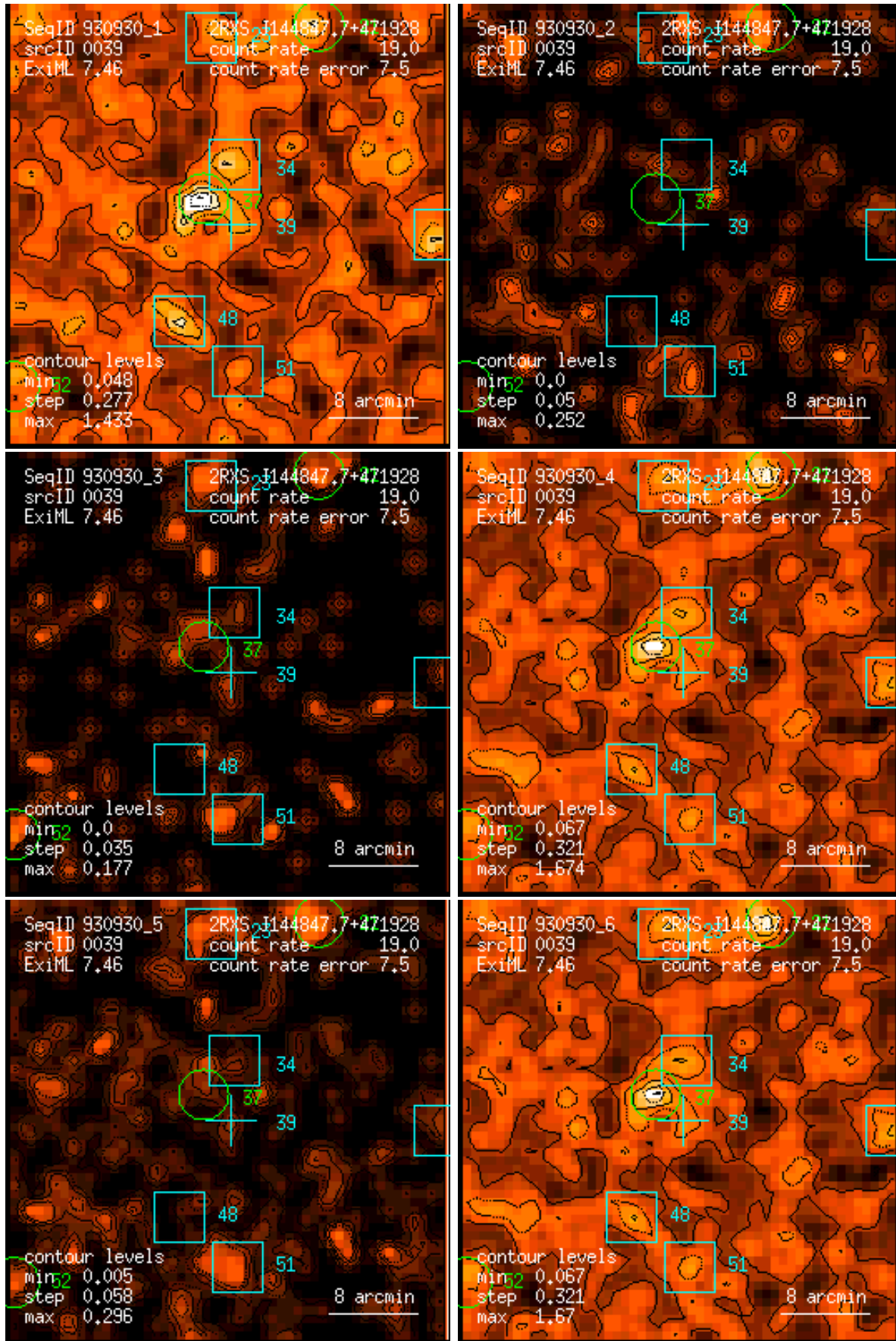
Figure 39: RASS 930930: detection 0039: band rate images, Gaussian filter: (1) PSPC channels 11 – 41, (2) 52 – 90, (3) 91 – 201, (4) 11 – 235, (5) 52 – 201, (6) 11 – 201. Broad band rates in counts/ks. Band rate contour levels in counts/ks/arcmin 2 .
