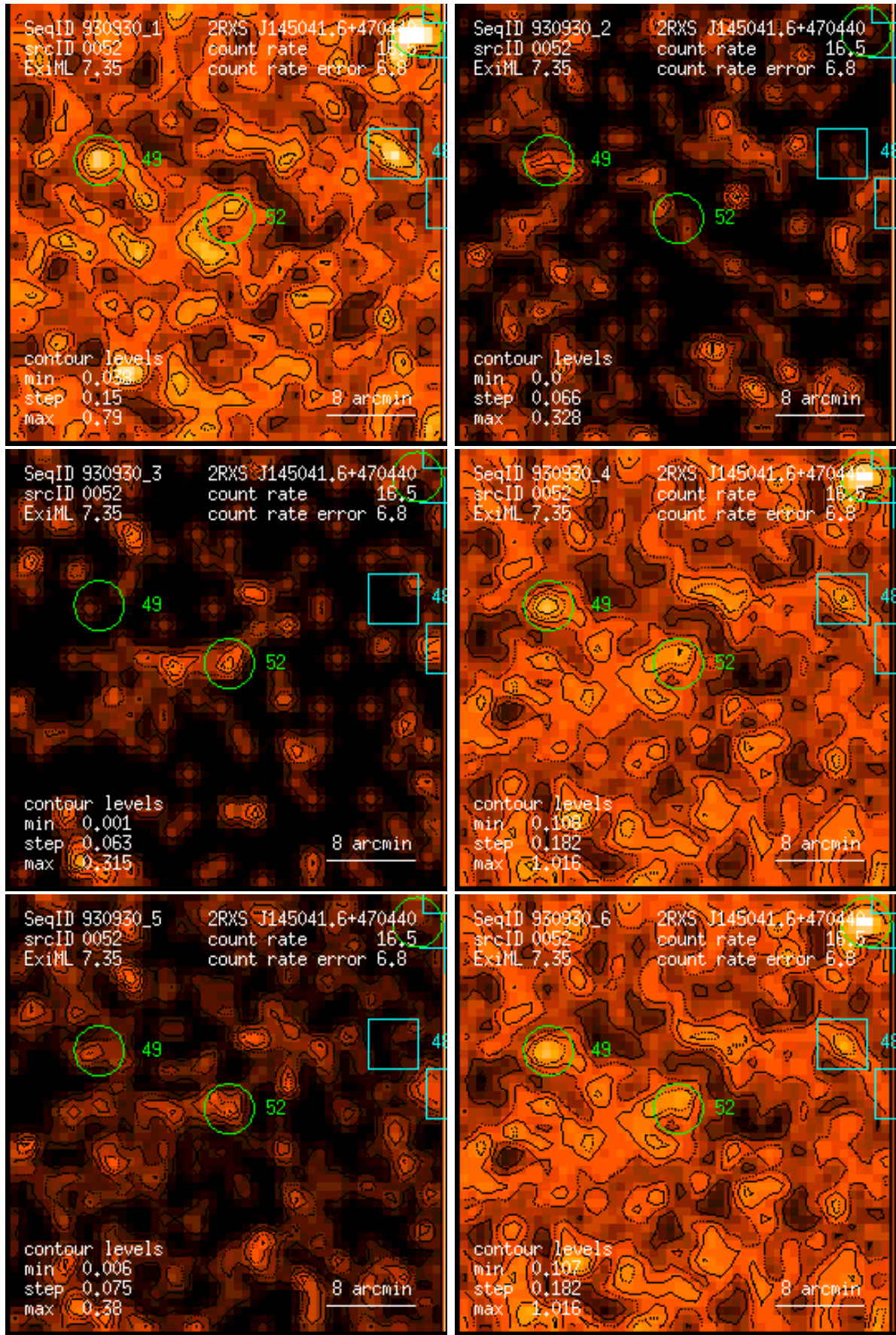
Figure 52: RASS 930930: detection 0052: band rate images, Gaussian filter: (1) PSPC channels 11 – 41, (2) 52 – 90, (3) 91 – 201, (4) 11 – 235, (5) 52 – 201, (6) 11 – 201. Broad band rates in counts/ks. Band rate contour levels in counts/ks/arcmin 2 .
