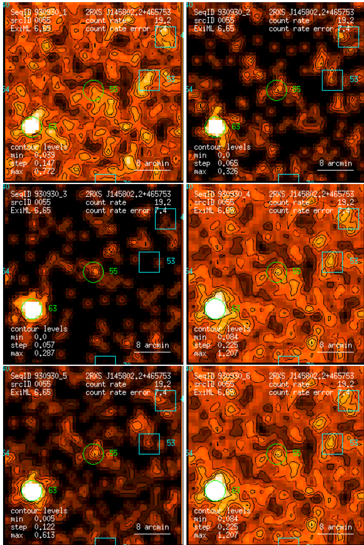
Figure 55: RASS 930930: detection 0055: band rate images, Gaussian filter: (1) PSPC channels 11 – 41, (2) 52 – 90, (3) 91 – 201, (4) 11 – 235, (5) 52 – 201, (6) 11 – 201. Broad band rates in counts/ks. Band rate contour levels in counts/ks/arcmin 2 .
