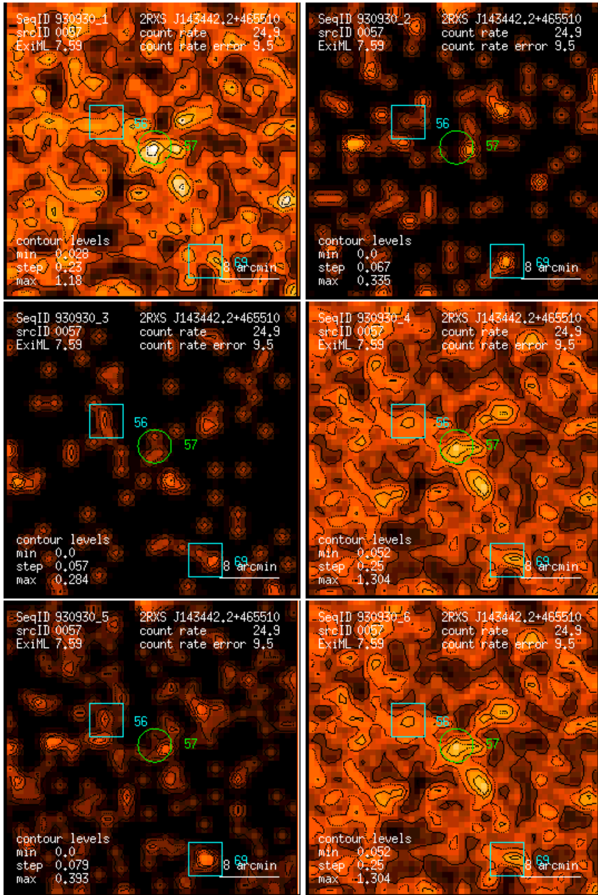
Figure 57: RASS 930930: detection 0057: band rate images, Gaussian filter: (1) PSPC channels 11 – 41, (2) 52 – 90, (3) 91 – 201, (4) 11 – 235, (5) 52 – 201, (6) 11 – 201. Broad band rates in counts/ks. Band rate contour levels in counts/ks/arcmin 2 .
