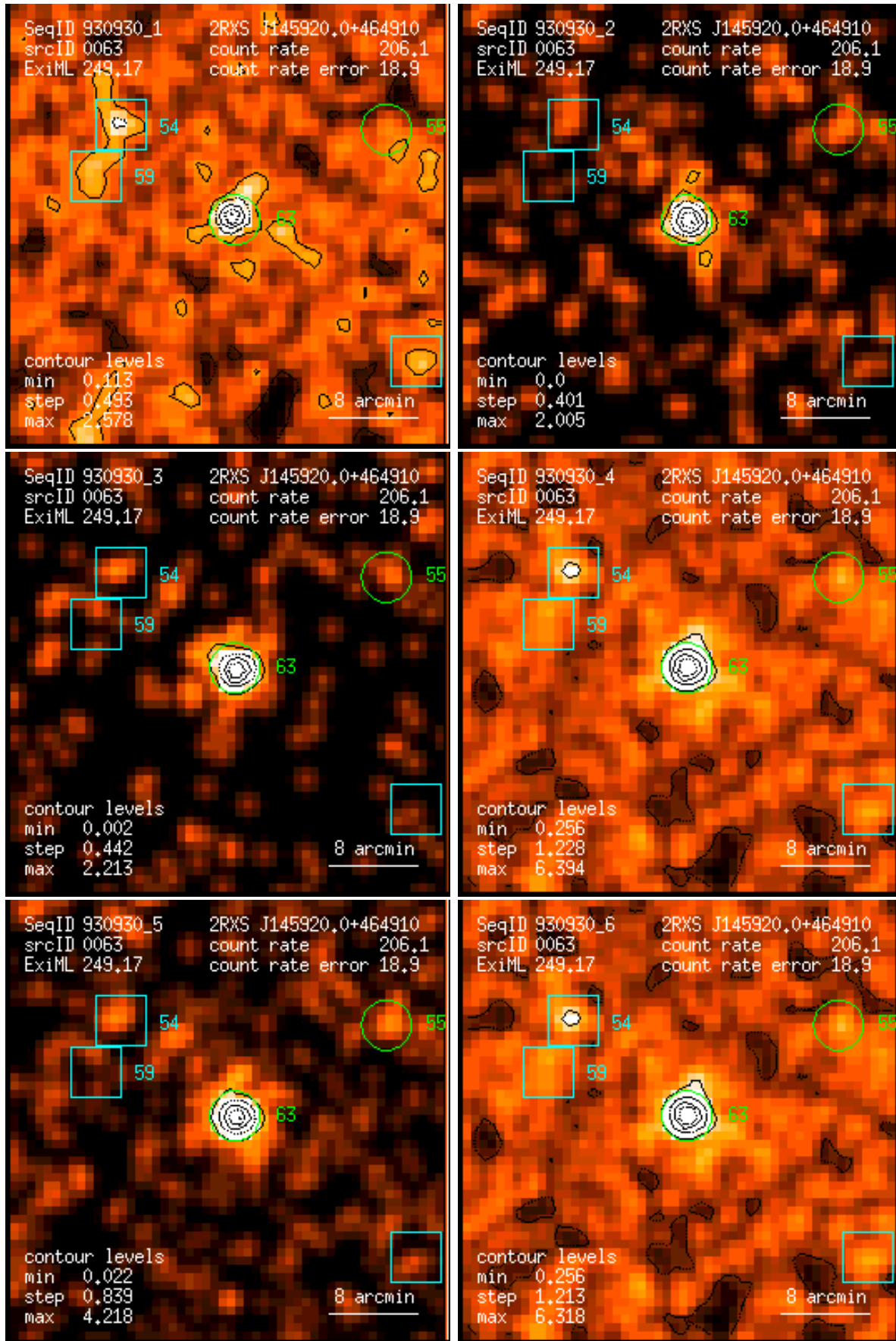
Figure 63: RASS 930930: detection 0063: band rate images, Gaussian filter: (1) PSPC channels 11 – 41, (2) 52 – 90, (3) 91 – 201, (4) 11 – 235, (5) 52 – 201, (6) 11 – 201. Broad band rates in counts/ks. Band rate contour levels in counts/ks/arcmin 2 .
