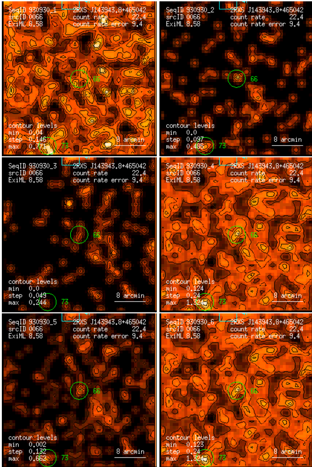
Figure 66: RASS 930930: detection 0066: band rate images, Gaussian filter: (1) PSPC channels 11 – 41, (2) 52 – 90, (3) 91 – 201, (4) 11 – 235, (5) 52 – 201, (6) 11 – 201. Broad band rates in counts/ks. Band rate contour levels in counts/ks/arcmin 2 .
