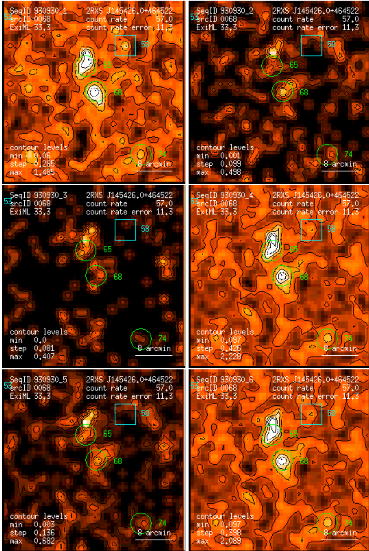
Figure 68: RASS 930930: detection 0068: band rate images, Gaussian filter: (1) PSPC channels 11 – 41, (2) 52 – 90, (3) 91 – 201, (4) 11 – 235, (5) 52 – 201, (6) 11 – 201. Broad band rates in counts/ks. Band rate contour levels in counts/ks/arcmin 2 .
