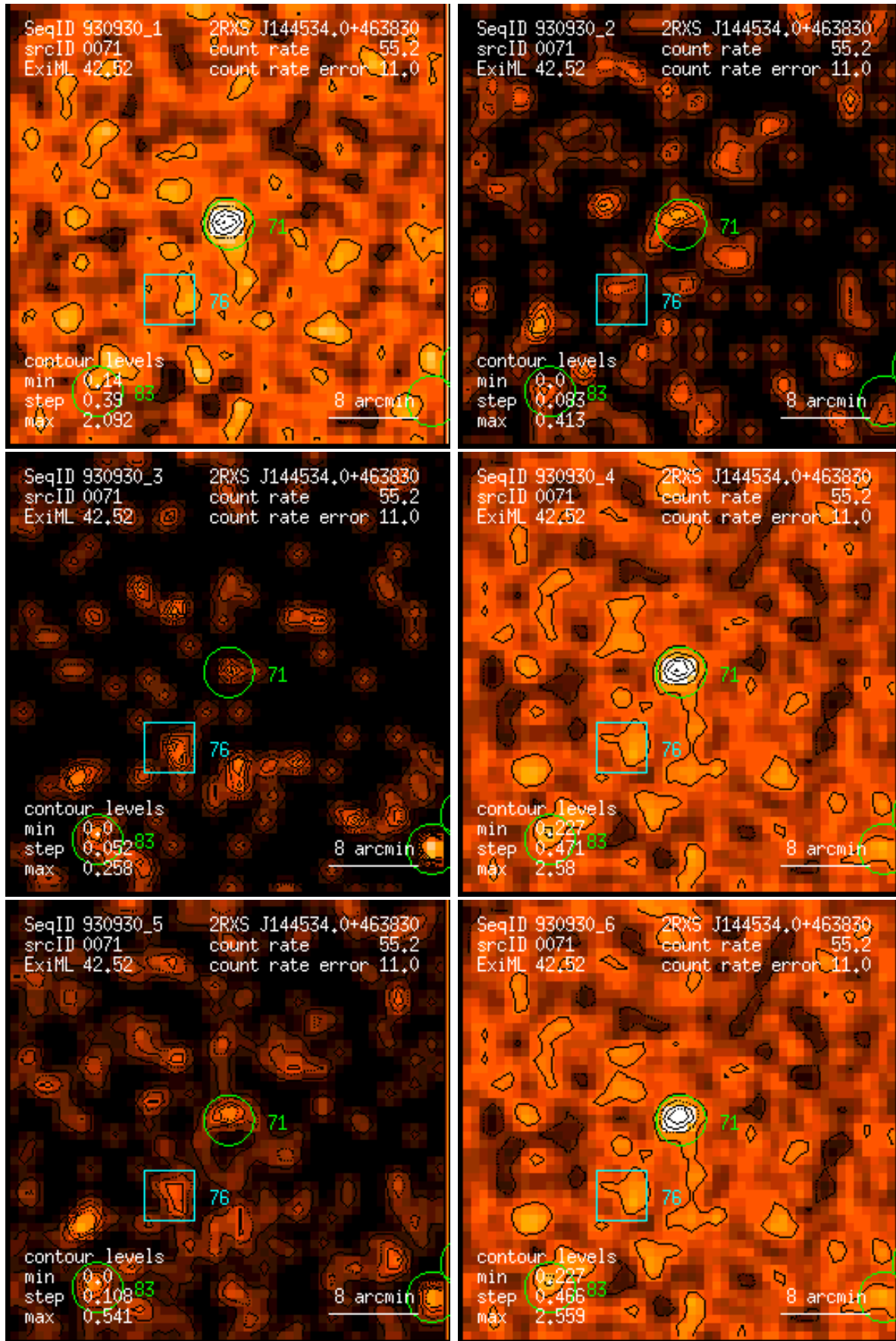
Figure 71: RASS 930930: detection 0071: band rate images, Gaussian filter: (1) PSPC channels 11 – 41, (2) 52 – 90, (3) 91 – 201, (4) 11 – 235, (5) 52 – 201, (6) 11 – 201. Broad band rates in counts/ks. Band rate contour levels in counts/ks/arcmin 2 .
