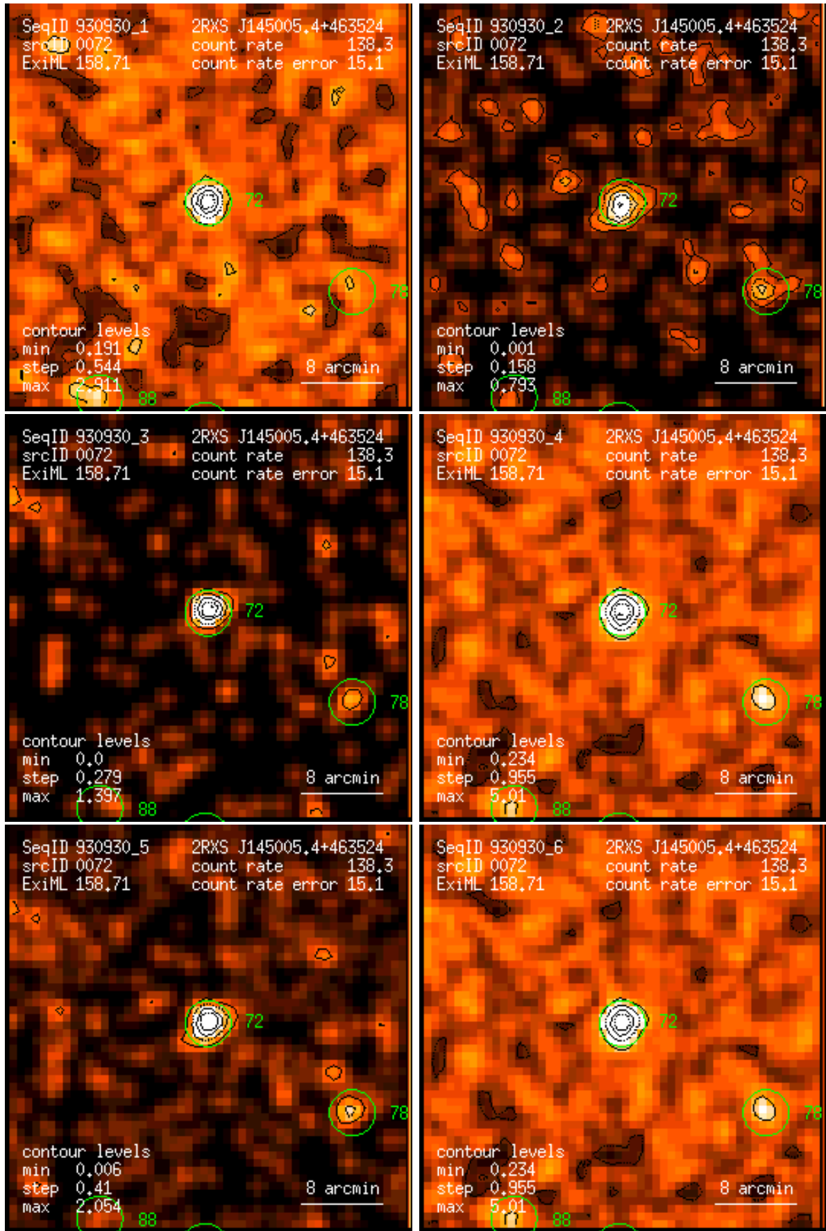
Figure 72: RASS 930930: detection 0072: band rate images, Gaussian filter: (1) PSPC channels 11 – 41, (2) 52 – 90, (3) 91 – 201, (4) 11 – 235, (5) 52 – 201, (6) 11 – 201. Broad band rates in counts/ks. Band rate contour levels in counts/ks/arcmin 2 .
