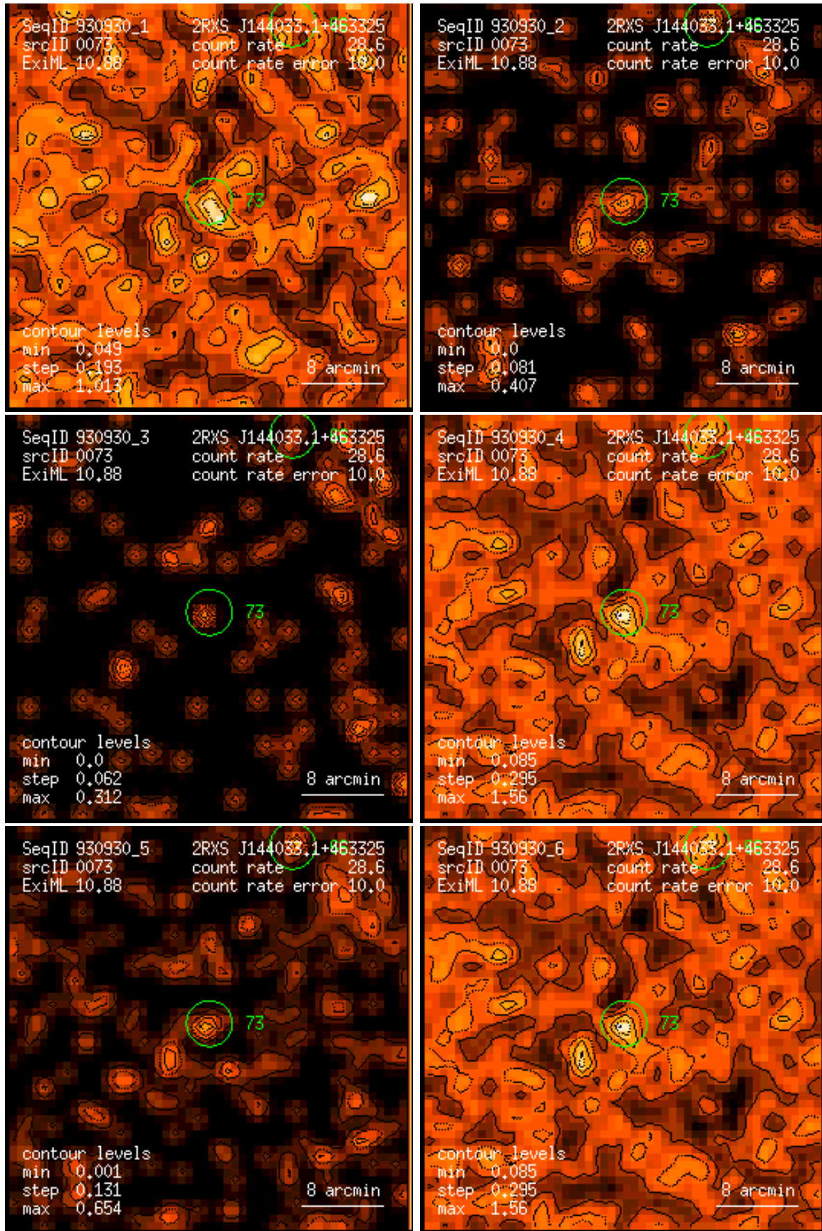
Figure 73: RASS 930930: detection 0073: band rate images, Gaussian filter: (1) PSPC channels 11 – 41, (2) 52 – 90, (3) 91 – 201, (4) 11 – 235, (5) 52 – 201, (6) 11 – 201. Broad band rates in counts/ks. Band rate contour levels in counts/ks/arcmin 2 .
