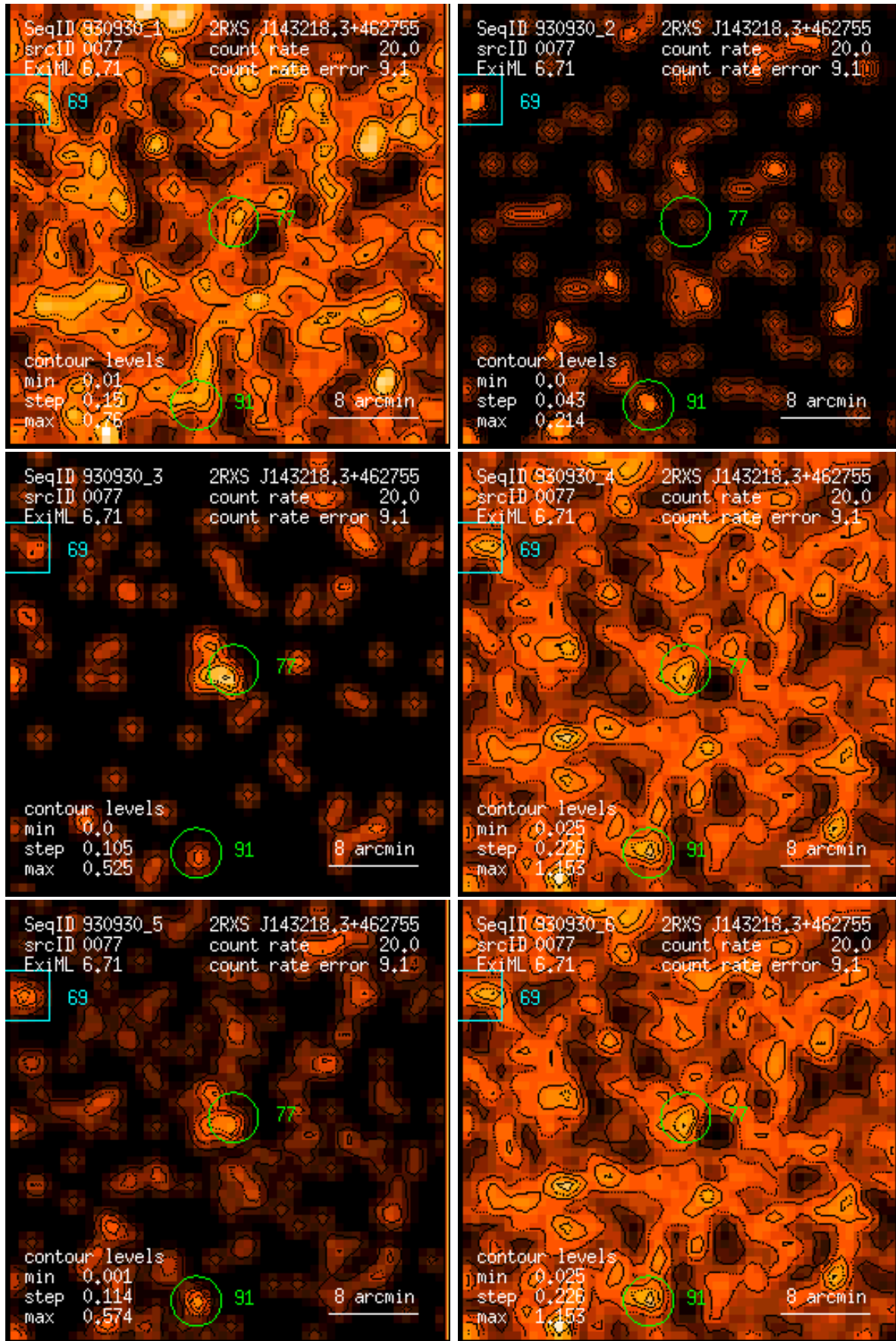
Figure 77: RASS 930930: detection 0077: band rate images, Gaussian filter: (1) PSPC channels 11 – 41, (2) 52 – 90, (3) 91 – 201, (4) 11 – 235, (5) 52 – 201, (6) 11 – 201. Broad band rates in counts/ks. Band rate contour levels in counts/ks/arcmin 2 .
