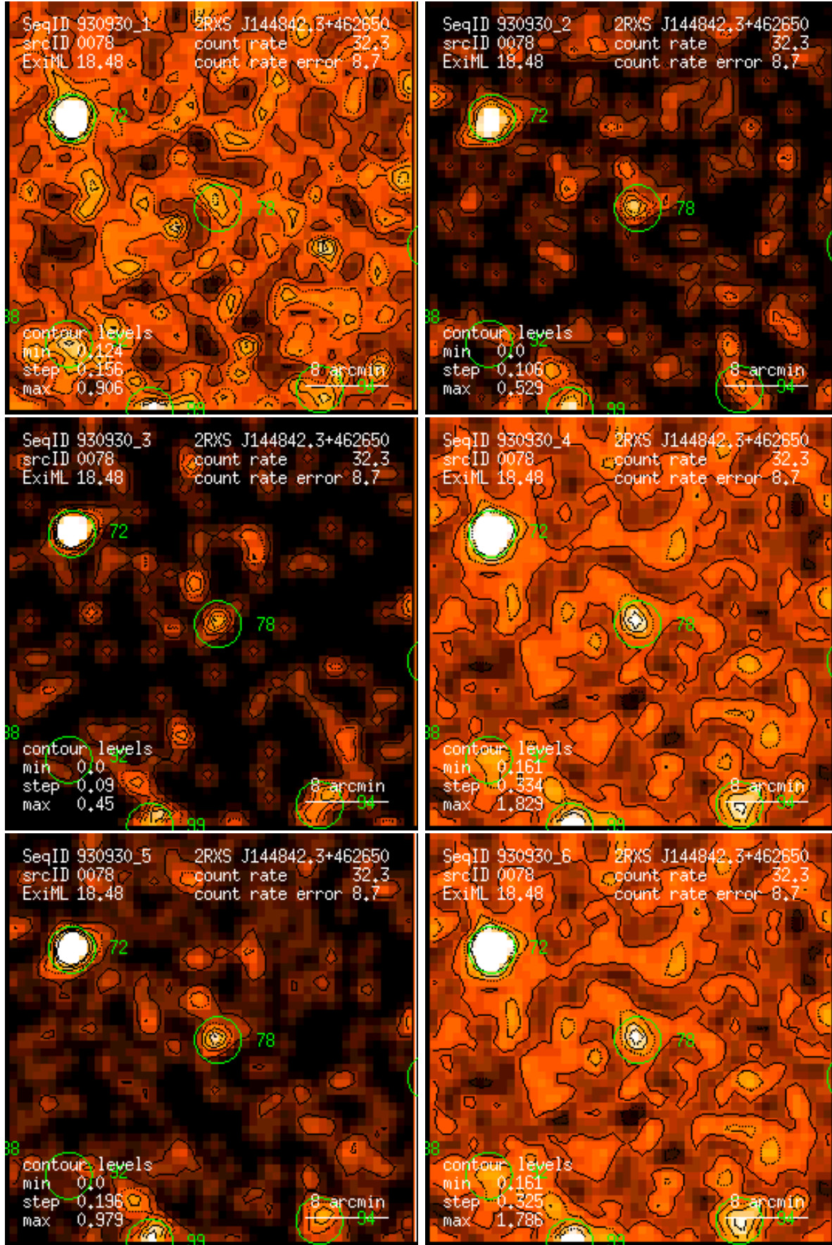
Figure 78: RASS 930930: detection 0078: band rate images, Gaussian filter: (1) PSPC channels 11 – 41, (2) 52 – 90, (3) 91 – 201, (4) 11 – 235, (5) 52 – 201, (6) 11 – 201. Broad band rates in counts/ks. Band rate contour levels in counts/ks/arcmin 2 .
