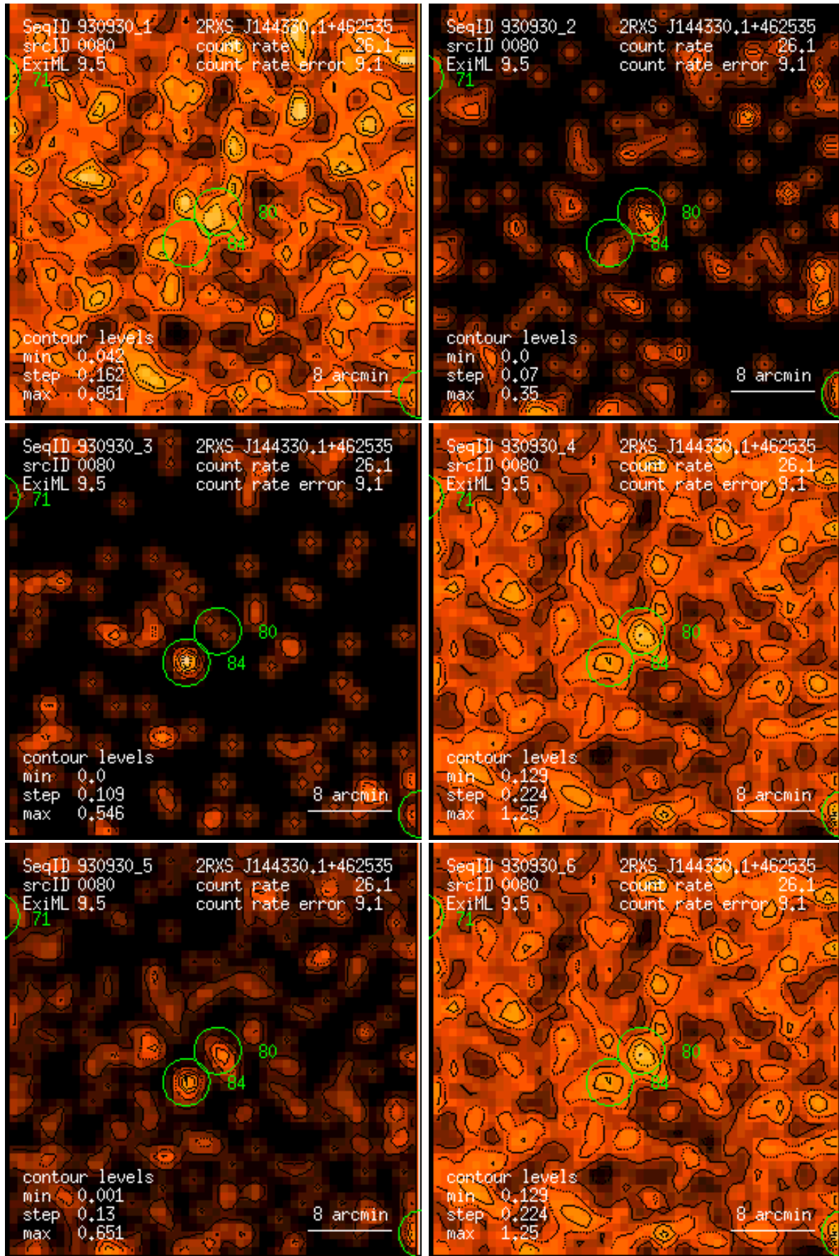
Figure 80: RASS 930930: detection 0080: band rate images, Gaussian filter: (1) PSPC channels 11 – 41, (2) 52 – 90, (3) 91 – 201, (4) 11 – 235, (5) 52 – 201, (6) 11 – 201. Broad band rates in counts/ks. Band rate contour levels in counts/ks/arcmin 2 .
