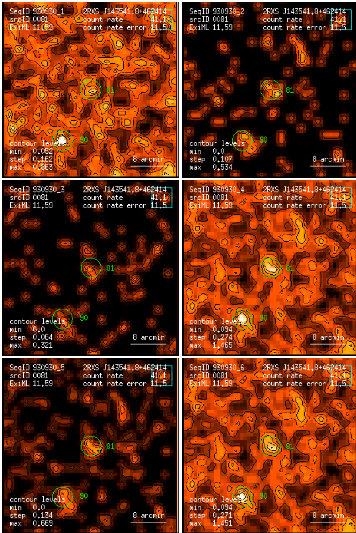
Figure 81: RASS 930930: detection 0081: band rate images, Gaussian filter: (1) PSPC channels 11 – 41, (2) 52 – 90, (3) 91 – 201, (4) 11 – 235, (5) 52 – 201, (6) 11 – 201. Broad band rates in counts/ks. Band rate contour levels in counts/ks/arcmin 2 .
