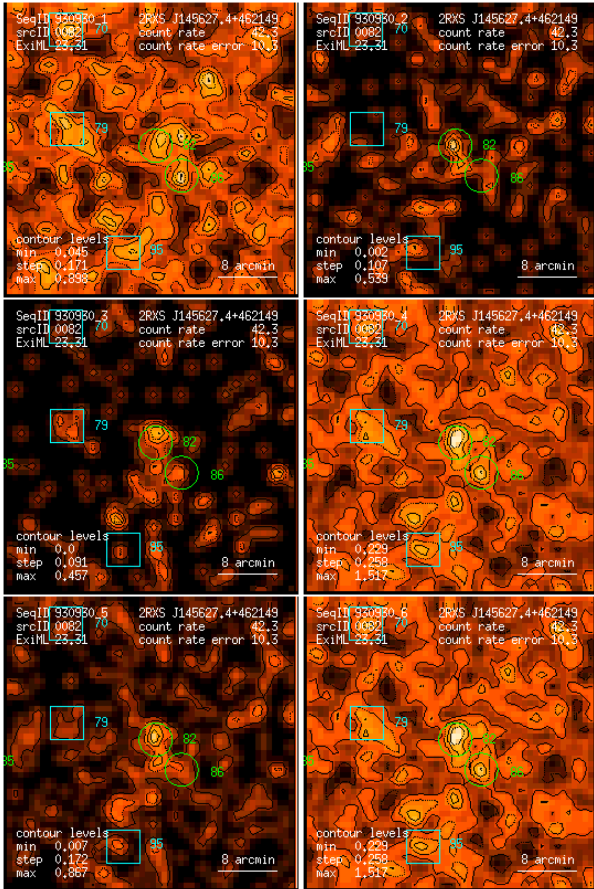
Figure 82: RASS 930930: detection 0082: band rate images, Gaussian filter: (1) PSPC channels 11 – 41, (2) 52 – 90, (3) 91 – 201, (4) 11 – 235, (5) 52 – 201, (6) 11 – 201. Broad band rates in counts/ks. Band rate contour levels in counts/ks/arcmin 2 .
