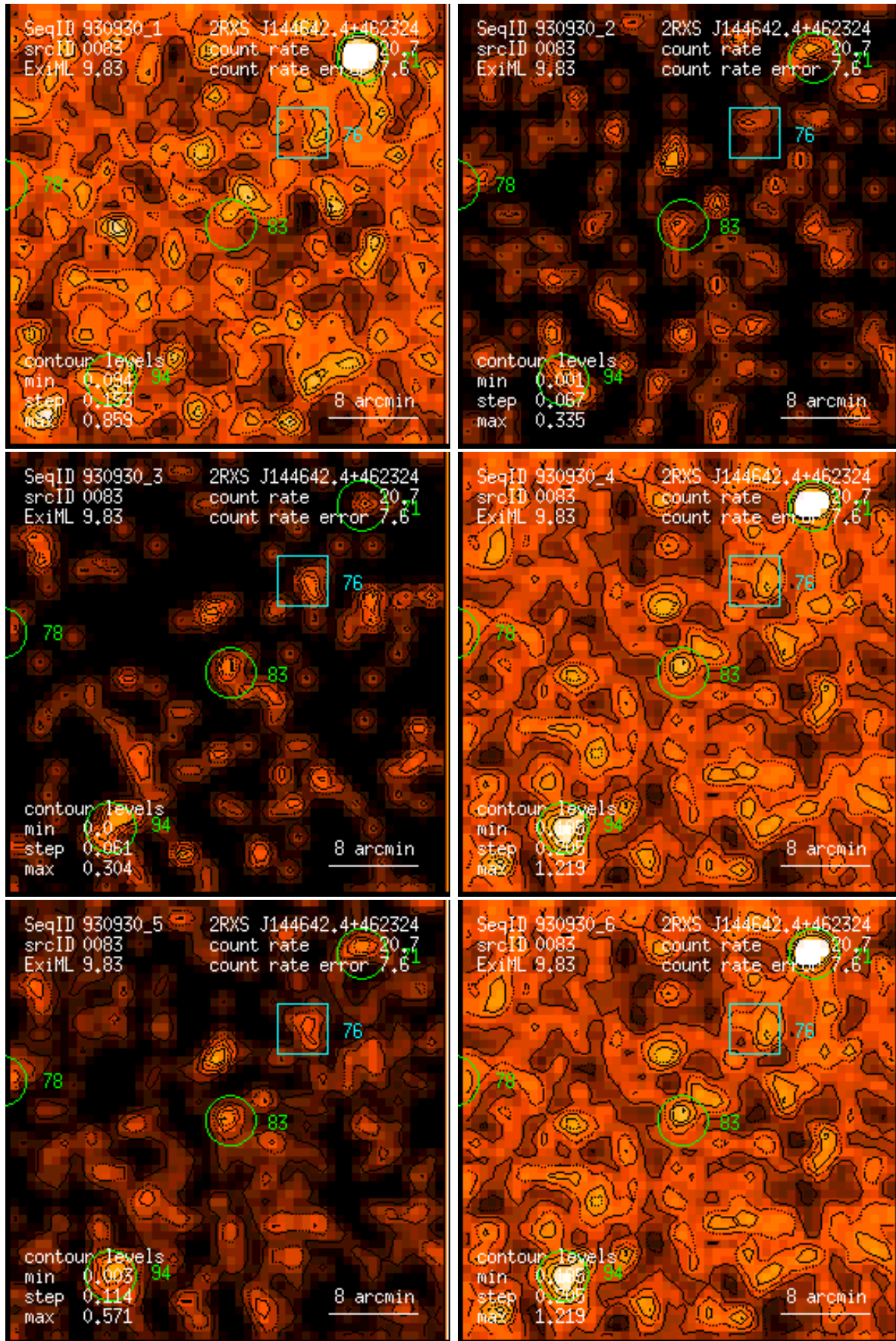
Figure 83: RASS 930930: detection 0083: band rate images, Gaussian filter: (1) PSPC channels 11 – 41, (2) 52 – 90, (3) 91 – 201, (4) 11 – 235, (5) 52 – 201, (6) 11 – 201. Broad band rates in counts/ks. Band rate contour levels in counts/ks/arcmin 2 .
