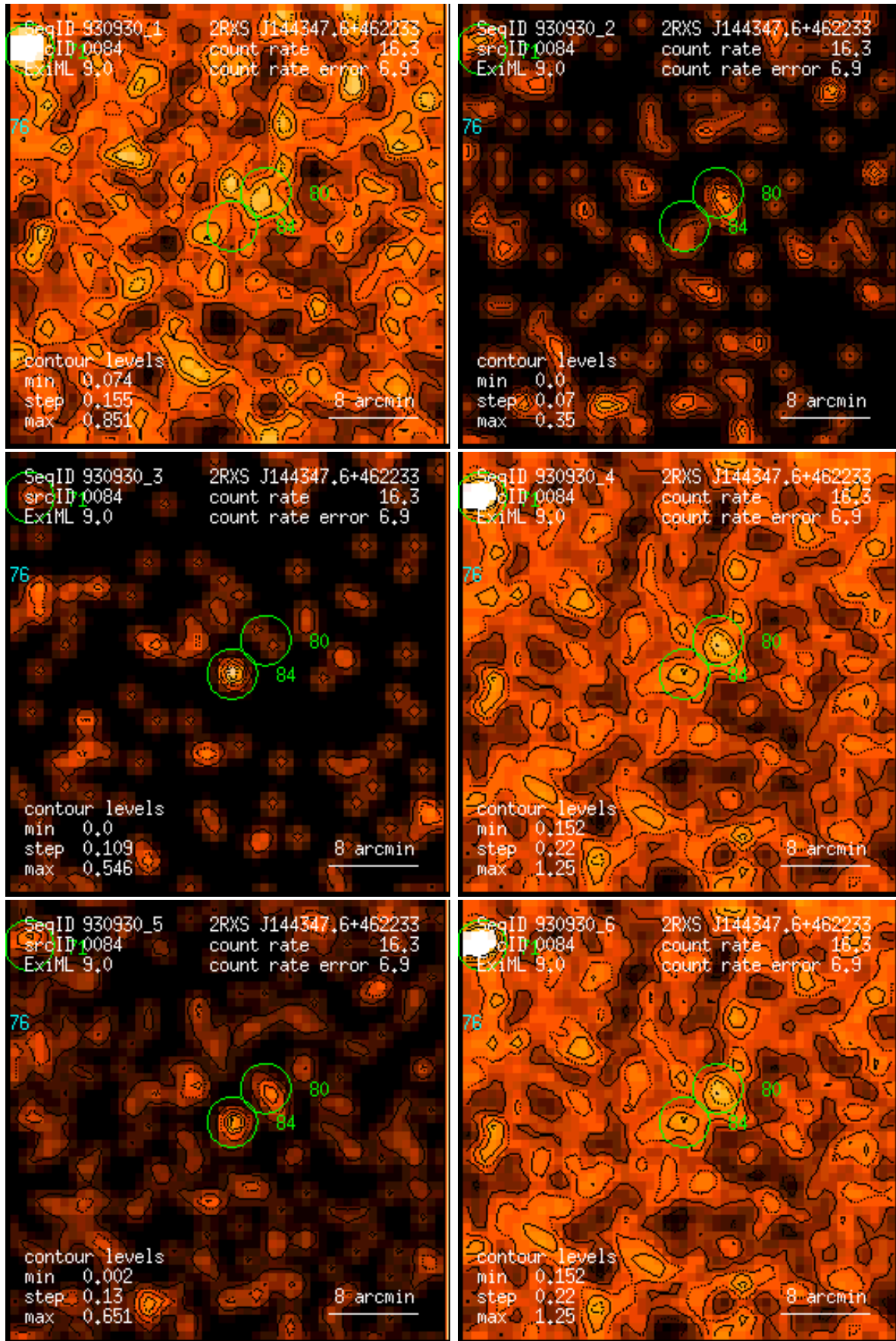
Figure 84: RASS 930930: detection 0084: band rate images, Gaussian filter: (1) PSPC channels 11 – 41, (2) 52 – 90, (3) 91 – 201, (4) 11 – 235, (5) 52 – 201, (6) 11 – 201. Broad band rates in counts/ks. Band rate contour levels in counts/ks/arcmin 2 .
