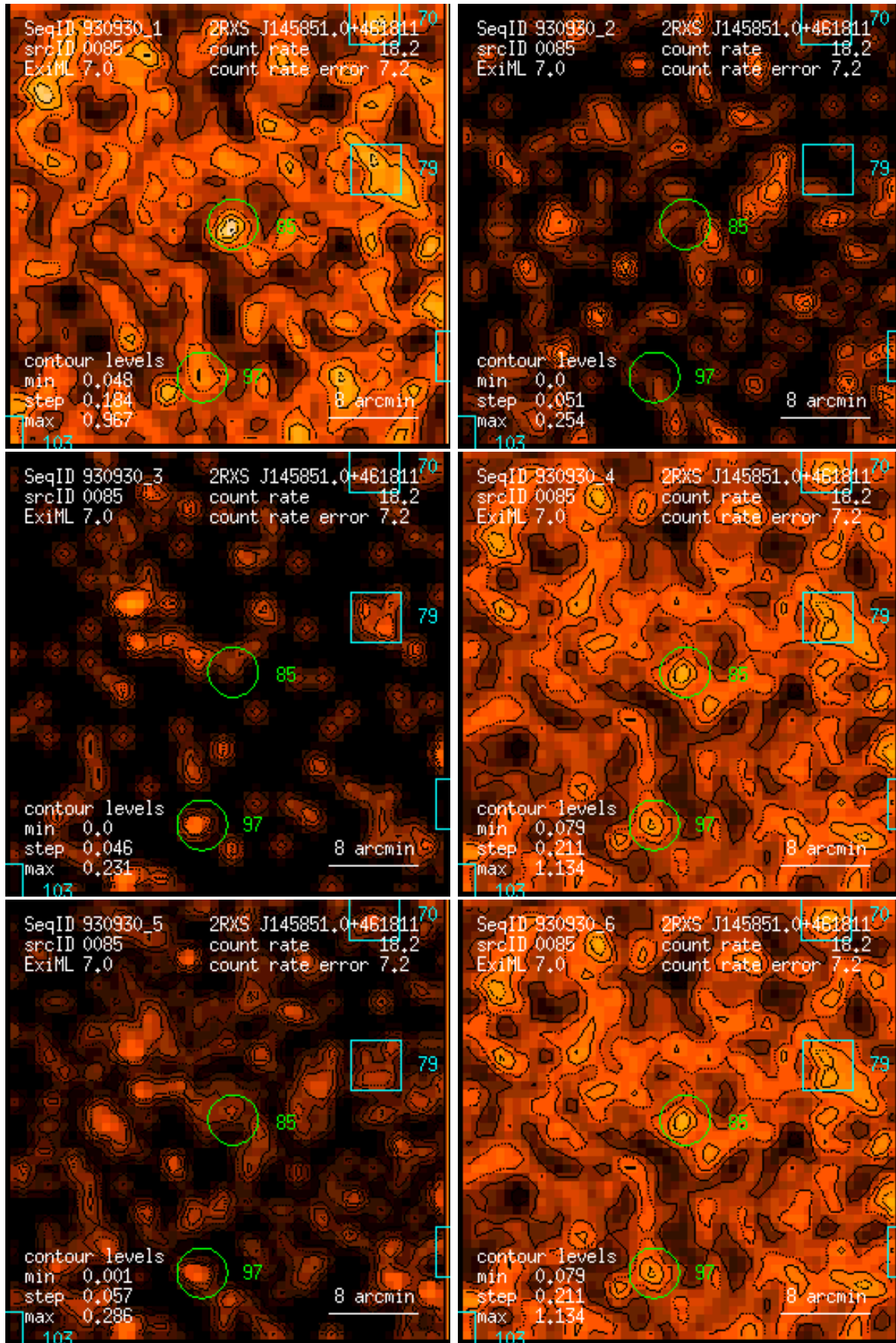
Figure 85: RASS 930930: detection 0085: band rate images, Gaussian filter: (1) PSPC channels 11 – 41, (2) 52 – 90, (3) 91 – 201, (4) 11 – 235, (5) 52 – 201, (6) 11 – 201. Broad band rates in counts/ks. Band rate contour levels in counts/ks/arcmin 2 .
