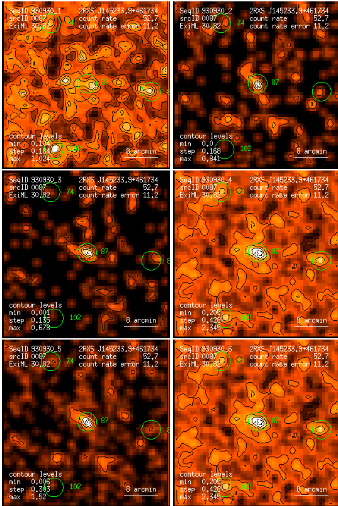
Figure 87: RASS 930930: detection 0087: band rate images, Gaussian filter: (1) PSPC channels 11 – 41, (2) 52 – 90, (3) 91 – 201, (4) 11 – 235, (5) 52 – 201, (6) 11 – 201. Broad band rates in counts/ks. Band rate contour levels in counts/ks/arcmin 2 .
