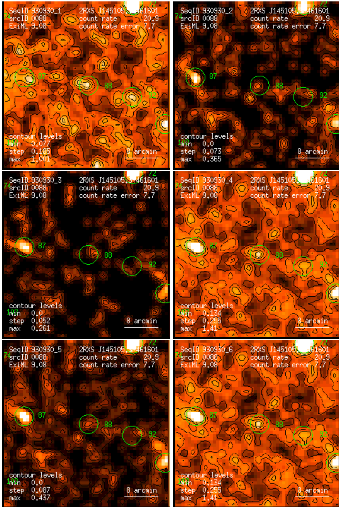
Figure 88: RASS 930930: detection 0088: band rate images, Gaussian filter: (1) PSPC channels 11 – 41, (2) 52 – 90, (3) 91 – 201, (4) 11 – 235, (5) 52 – 201, (6) 11 – 201. Broad band rates in counts/ks. Band rate contour levels in counts/ks/arcmin 2 .
