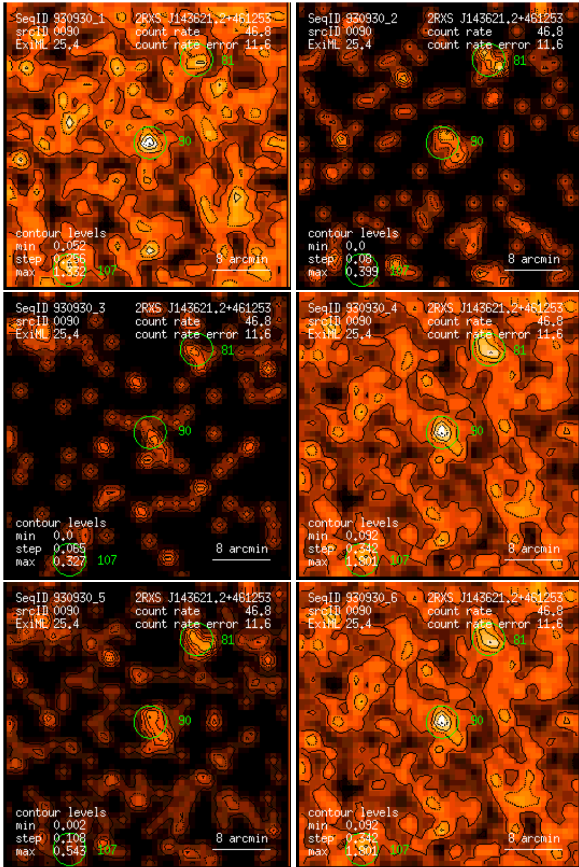
Figure 90: RASS 930930: detection 0090: band rate images, Gaussian filter: (1) PSPC channels 11 – 41, (2) 52 – 90, (3) 91 – 201, (4) 11 – 235, (5) 52 – 201, (6) 11 – 201. Broad band rates in counts/ks. Band rate contour levels in counts/ks/arcmin 2 .
