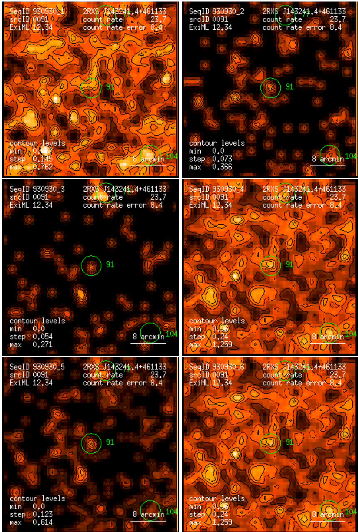
Figure 91: RASS 930930: detection 0091: band rate images, Gaussian filter: (1) PSPC channels 11 – 41, (2) 52 – 90, (3) 91 – 201, (4) 11 – 235, (5) 52 – 201, (6) 11 – 201. Broad band rates in counts/ks. Band rate contour levels in counts/ks/arcmin 2 .
