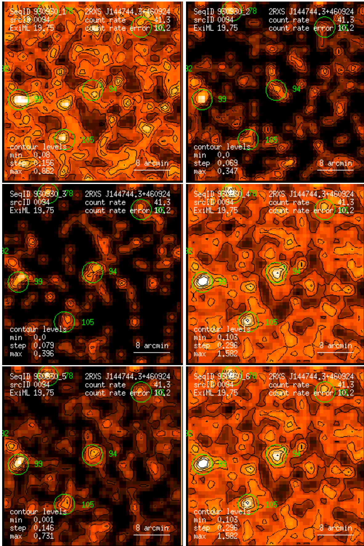
Figure 94: RASS 930930: detection 0094: band rate images, Gaussian filter: (1) PSPC channels 11 – 41, (2) 52 – 90, (3) 91 – 201, (4) 11 – 235, (5) 52 – 201, (6) 11 – 201. Broad band rates in counts/ks. Band rate contour levels in counts/ks/arcmin 2 .
