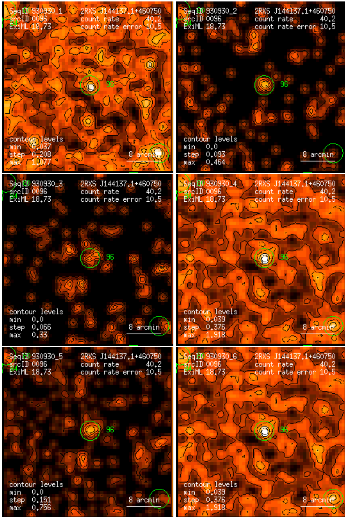
Figure 96: RASS 930930: detection 0096: band rate images, Gaussian filter: (1) PSPC channels 11 – 41, (2) 52 – 90, (3) 91 – 201, (4) 11 – 235, (5) 52 – 201, (6) 11 – 201. Broad band rates in counts/ks. Band rate contour levels in counts/ks/arcmin 2 .
