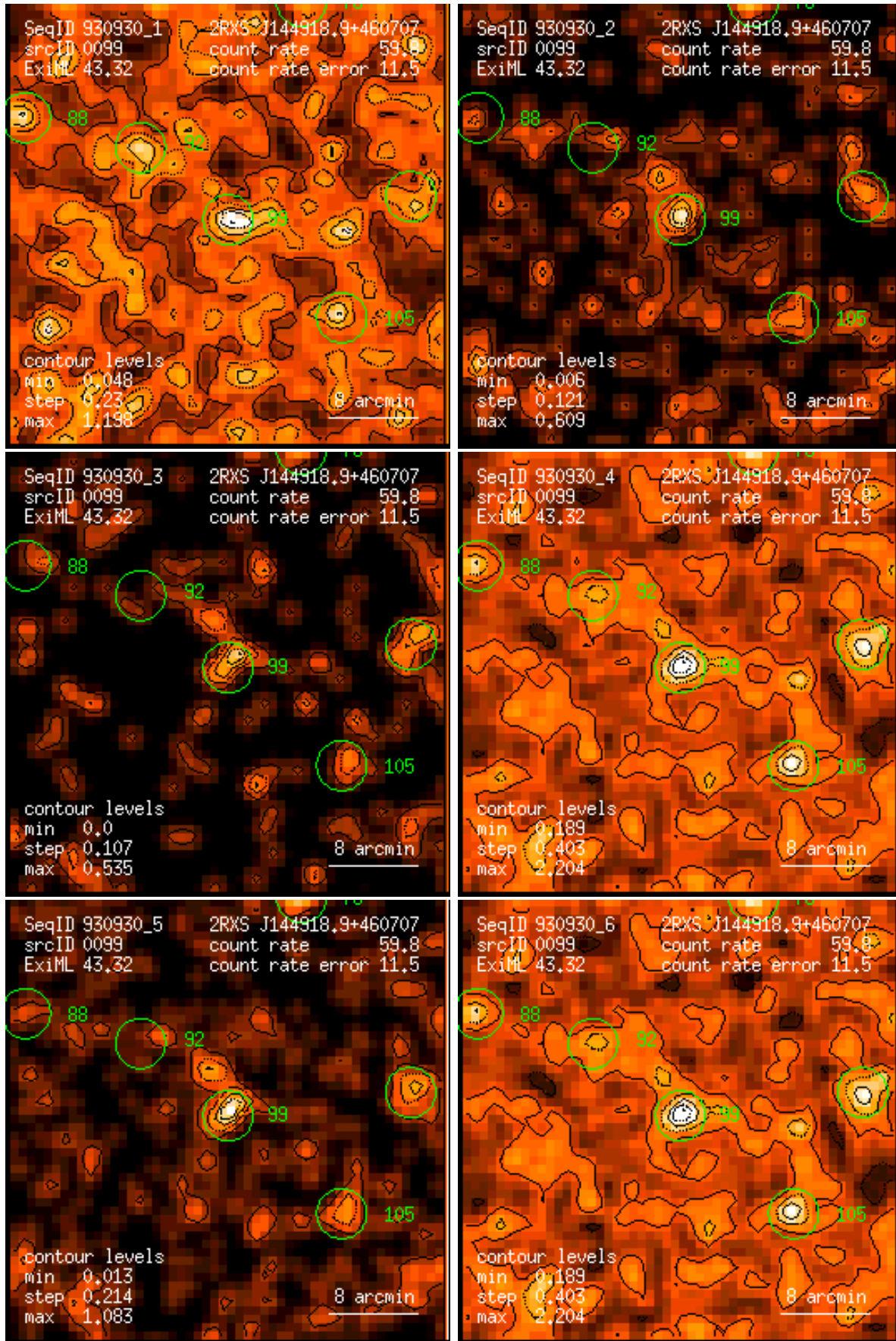
Figure 99: RASS 930930: detection 0099: band rate images, Gaussian filter: (1) PSPC channels 11 – 41, (2) 52 – 90, (3) 91 – 201, (4) 11 – 235, (5) 52 – 201, (6) 11 – 201. Broad band rates in counts/ks. Band rate contour levels in counts/ks/arcmin 2 .
