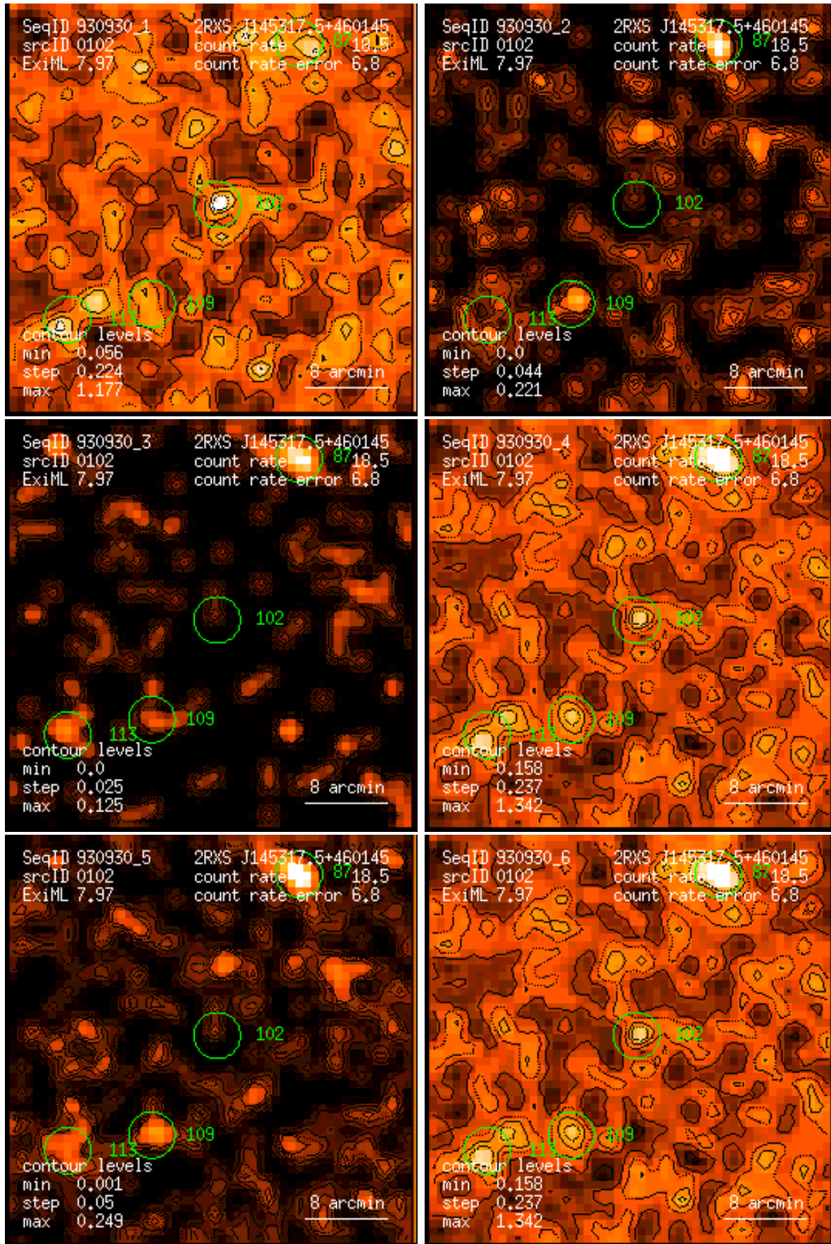
Figure 102: RASS 930930: detection 0102: band rate images, Gaussian filter: (1) PSPC channels 11 – 41, (2) 52 – 90, (3) 91 – 201, (4) 11 – 235, (5) 52 – 201, (6) 11 – 201. Broad band rates in counts/ks. Band rate contour levels in counts/ks/arcmin 2 .
