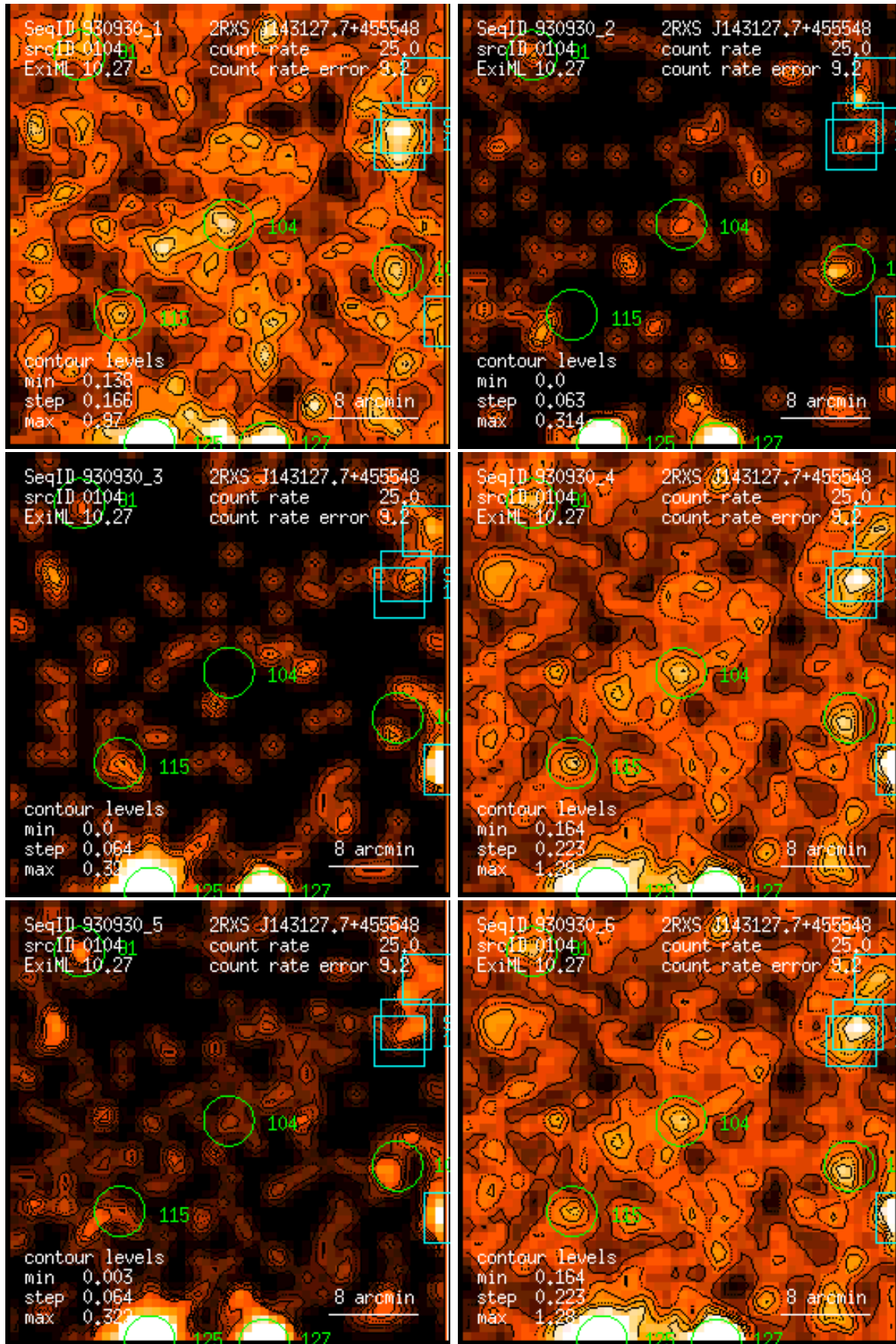
Figure 104: RASS 930930: detection 0104: band rate images, Gaussian filter: (1) PSPC channels 11 – 41, (2) 52 – 90, (3) 91 – 201, (4) 11 – 235, (5) 52 – 201, (6) 11 – 201. Broad band rates in counts/ks. Band rate contour levels in counts/ks/arcmin 2 .
