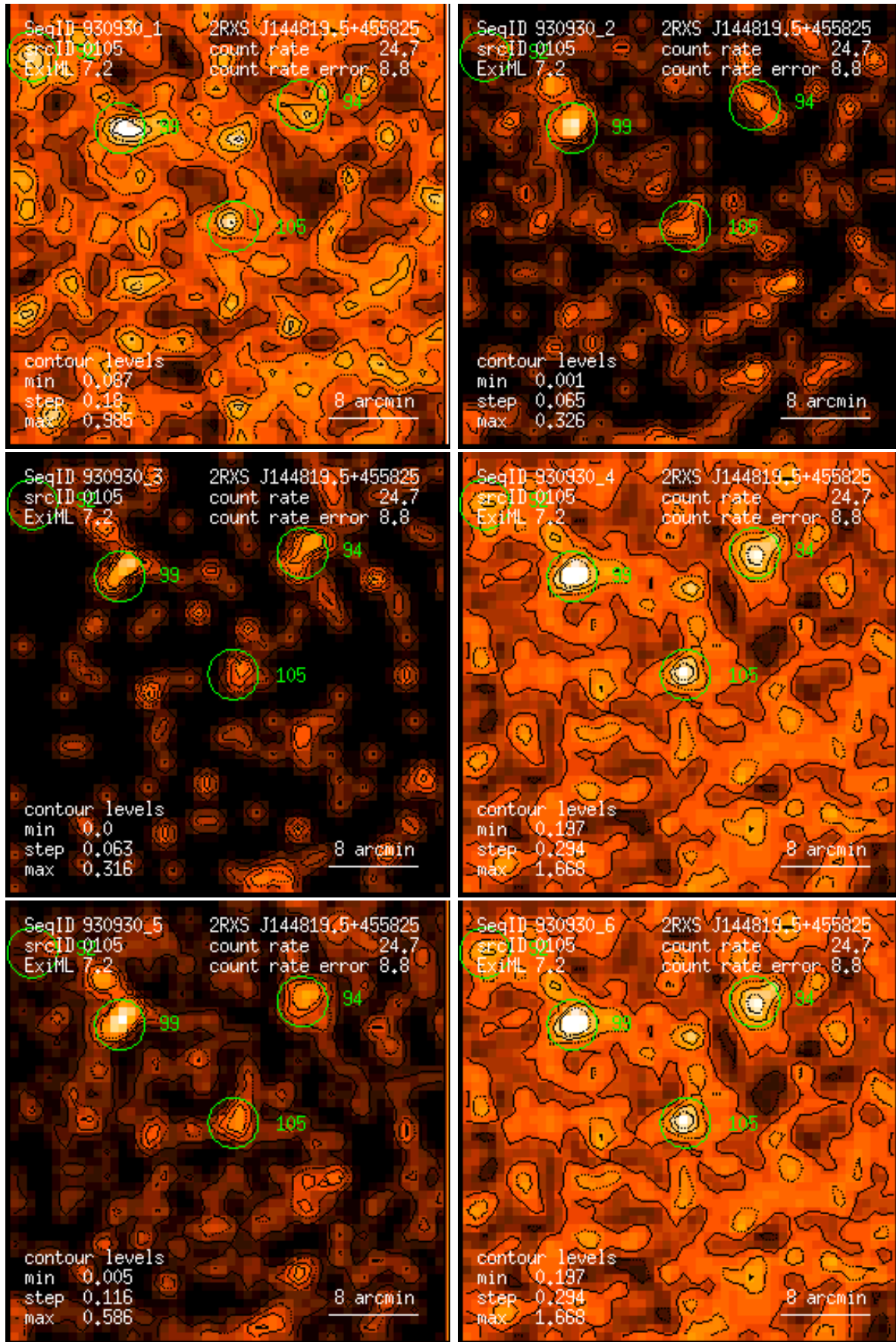
Figure 105: RASS 930930: detection 0105: band rate images, Gaussian filter: (1) PSPC channels 11 – 41, (2) 52 – 90, (3) 91 – 201, (4) 11 – 235, (5) 52 – 201, (6) 11 – 201. Broad band rates in counts/ks. Band rate contour levels in counts/ks/arcmin 2 .
