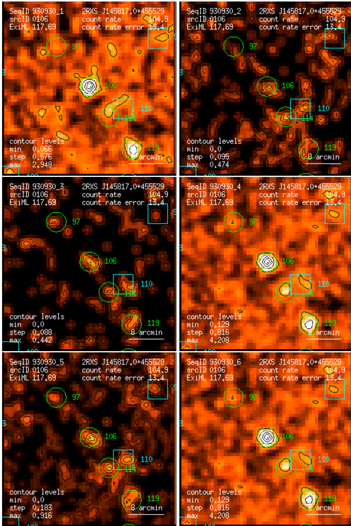
Figure 106: RASS 930930: detection 0106: band rate images, Gaussian filter: (1) PSPC channels 11 – 41, (2) 52 – 90, (3) 91 – 201, (4) 11 – 235, (5) 52 – 201, (6) 11 – 201. Broad band rates in counts/ks. Band rate contour levels in counts/ks/arcmin 2 .
