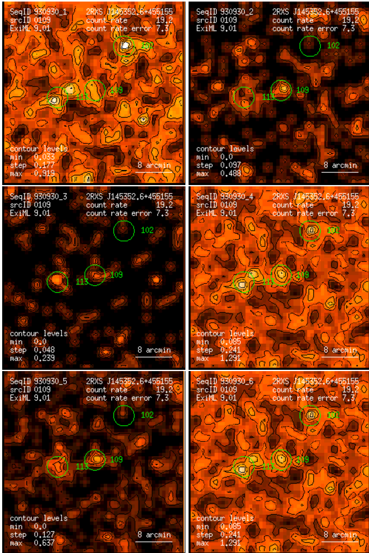
Figure 109: RASS 930930: detection 0109: band rate images, Gaussian filter: (1) PSPC channels 11 – 41, (2) 52 – 90, (3) 91 – 201, (4) 11 – 235, (5) 52 – 201, (6) 11 – 201. Broad band rates in counts/ks. Band rate contour levels in counts/ks/arcmin 2 .
