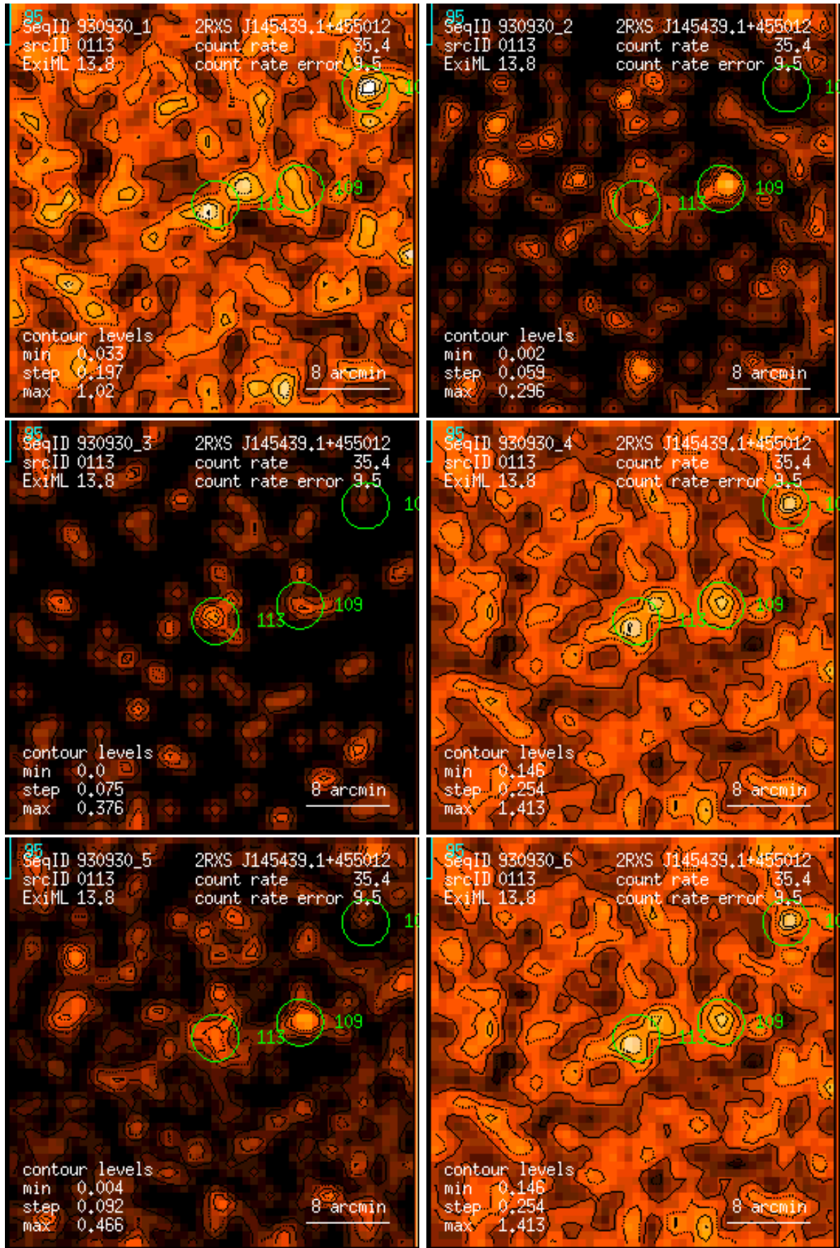
Figure 113: RASS 930930: detection 0113: band rate images, Gaussian filter: (1) PSPC channels 11 – 41, (2) 52 – 90, (3) 91 – 201, (4) 11 – 235, (5) 52 – 201, (6) 11 – 201. Broad band rates in counts/ks. Band rate contour levels in counts/ks/arcmin 2 .
