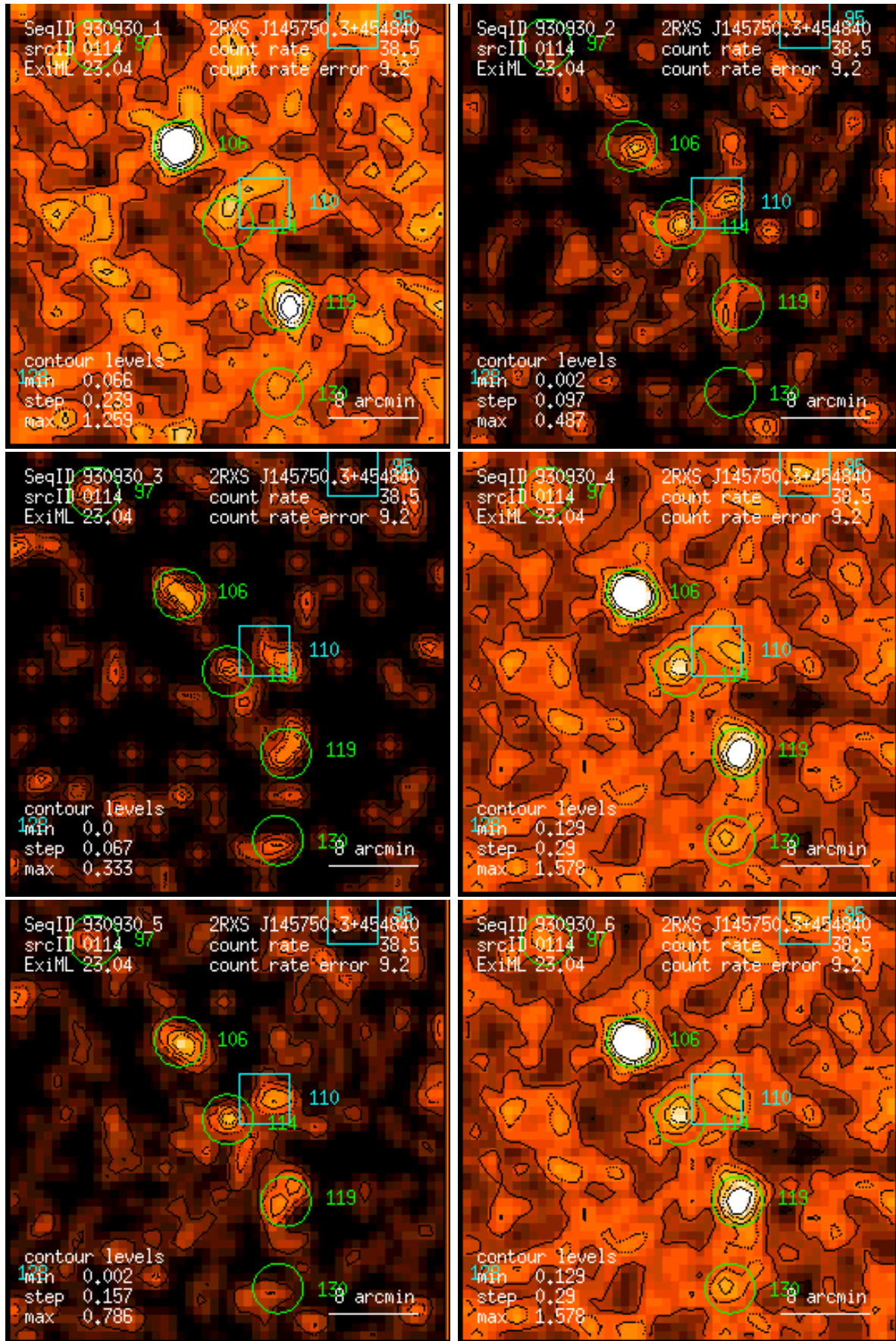
Figure 114: RASS 930930: detection 0114: band rate images, Gaussian filter: (1) PSPC channels 11 – 41, (2) 52 – 90, (3) 91 – 201, (4) 11 – 235, (5) 52 – 201, (6) 11 – 201. Broad band rates in counts/ks. Band rate contour levels in counts/ks/arcmin 2 .
