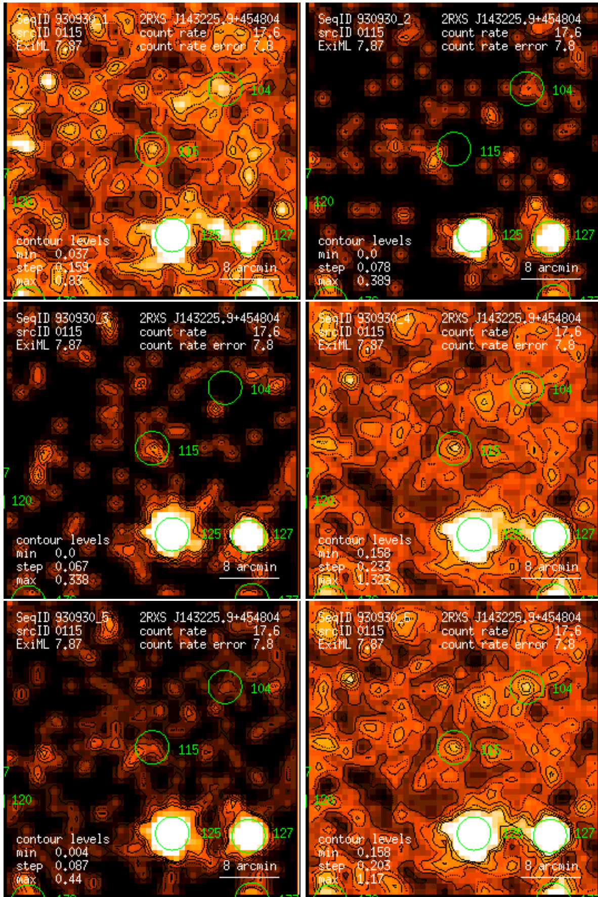
Figure 115: RASS 930930: detection 0115: band rate images, Gaussian filter: (1) PSPC channels 11 – 41, (2) 52 – 90, (3) 91 – 201, (4) 11 – 235, (5) 52 – 201, (6) 11 – 201. Broad band rates in counts/ks. Band rate contour levels in counts/ks/arcmin 2 .
