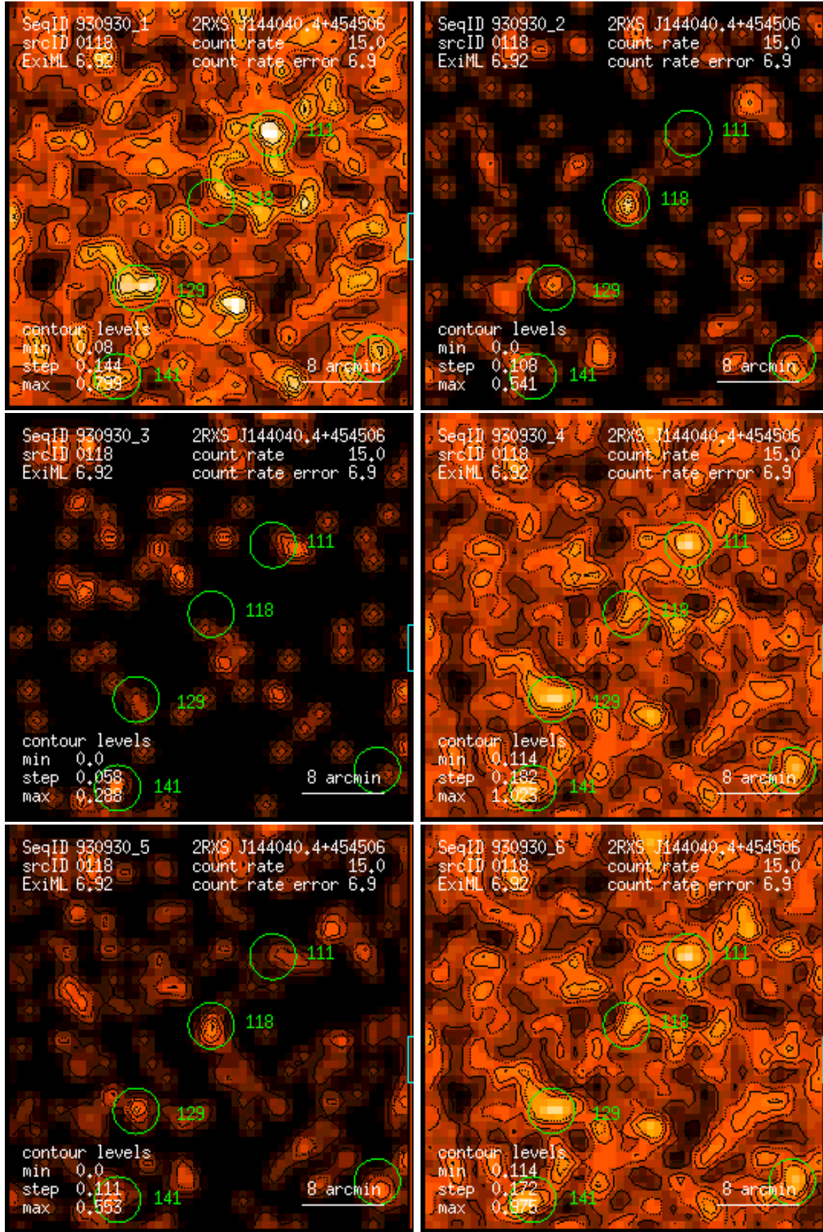
Figure 118: RASS 930930: detection 0118: band rate images, Gaussian filter: (1) PSPC channels 11 – 41, (2) 52 – 90, (3) 91 – 201, (4) 11 – 235, (5) 52 – 201, (6) 11 – 201. Broad band rates in counts/ks. Band rate contour levels in counts/ks/arcmin 2 .
