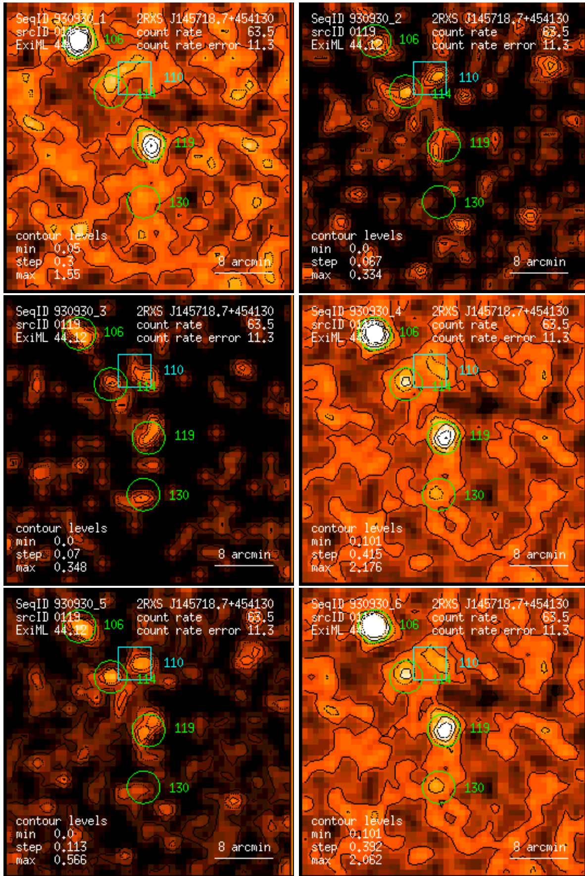
Figure 119: RASS 930930: detection 0119: band rate images, Gaussian filter: (1) PSPC channels 11 – 41, (2) 52 – 90, (3) 91 – 201, (4) 11 – 235, (5) 52 – 201, (6) 11 – 201. Broad band rates in counts/ks. Band rate contour levels in counts/ks/arcmin 2 .
