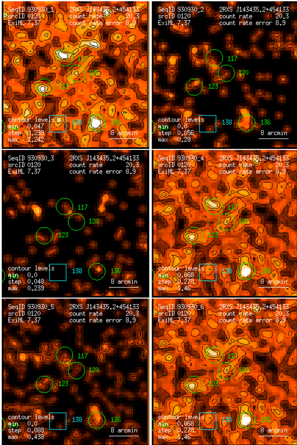
Figure 120: RASS 930930: detection 0120: band rate images, Gaussian filter: (1) PSPC channels 11 – 41, (2) 52 – 90, (3) 91 – 201, (4) 11 – 235, (5) 52 – 201, (6) 11 – 201. Broad band rates in counts/ks. Band rate contour levels in counts/ks/arcmin 2 .
