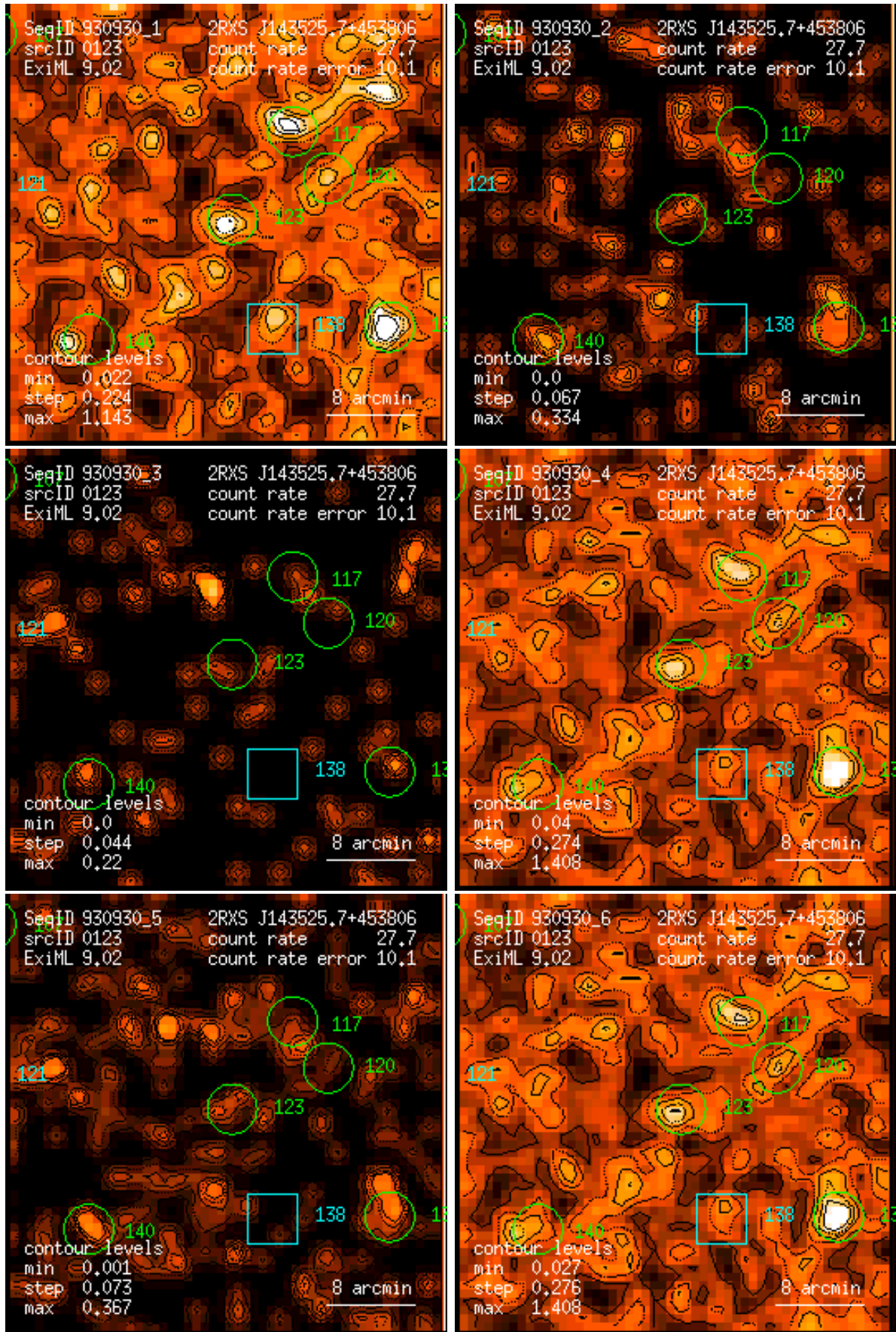
Figure 123: RASS 930930: detection 0123: band rate images, Gaussian filter: (1) PSPC channels 11 – 41, (2) 52 – 90, (3) 91 – 201, (4) 11 – 235, (5) 52 – 201, (6) 11 – 201. Broad band rates in counts/ks. Band rate contour levels in counts/ks/arcmin 2 .
