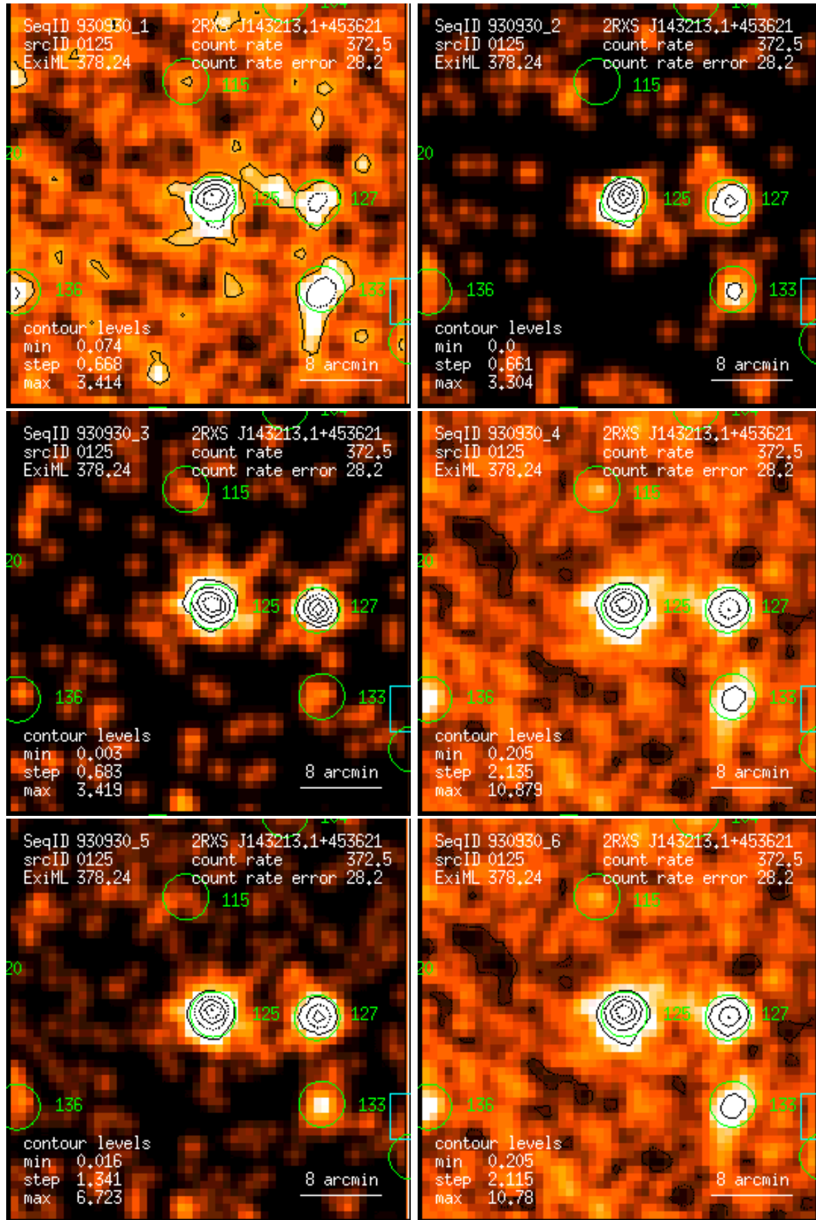
Figure 125: RASS 930930: detection 0125: band rate images, Gaussian filter: (1) PSPC channels 11 – 41, (2) 52 – 90, (3) 91 – 201, (4) 11 – 235, (5) 52 – 201, (6) 11 – 201. Broad band rates in counts/ks. Band rate contour levels in counts/ks/arcmin 2 .
