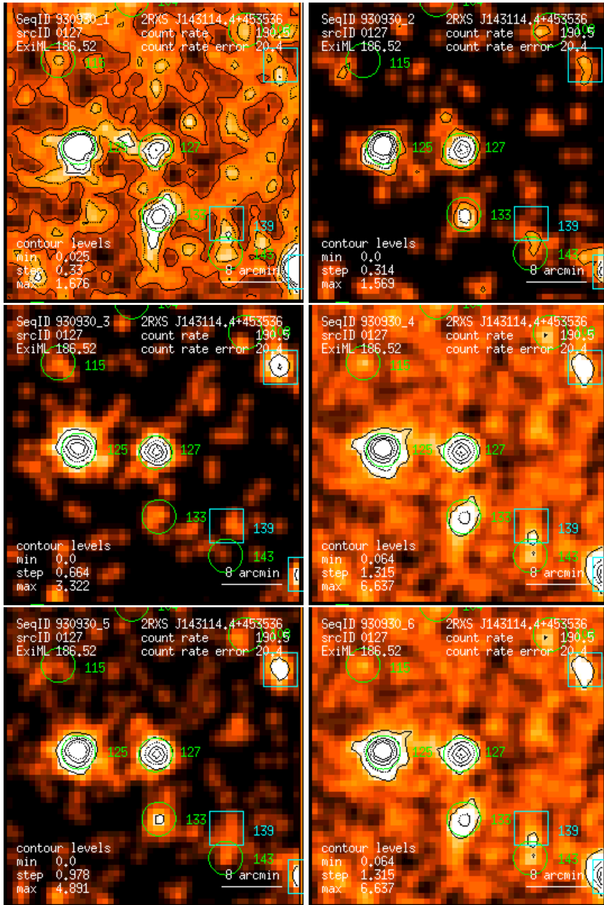
Figure 127: RASS 930930: detection 0127: band rate images, Gaussian filter: (1) PSPC channels 11 – 41, (2) 52 – 90, (3) 91 – 201, (4) 11 – 235, (5) 52 – 201, (6) 11 – 201. Broad band rates in counts/ks. Band rate contour levels in counts/ks/arcmin 2 .
