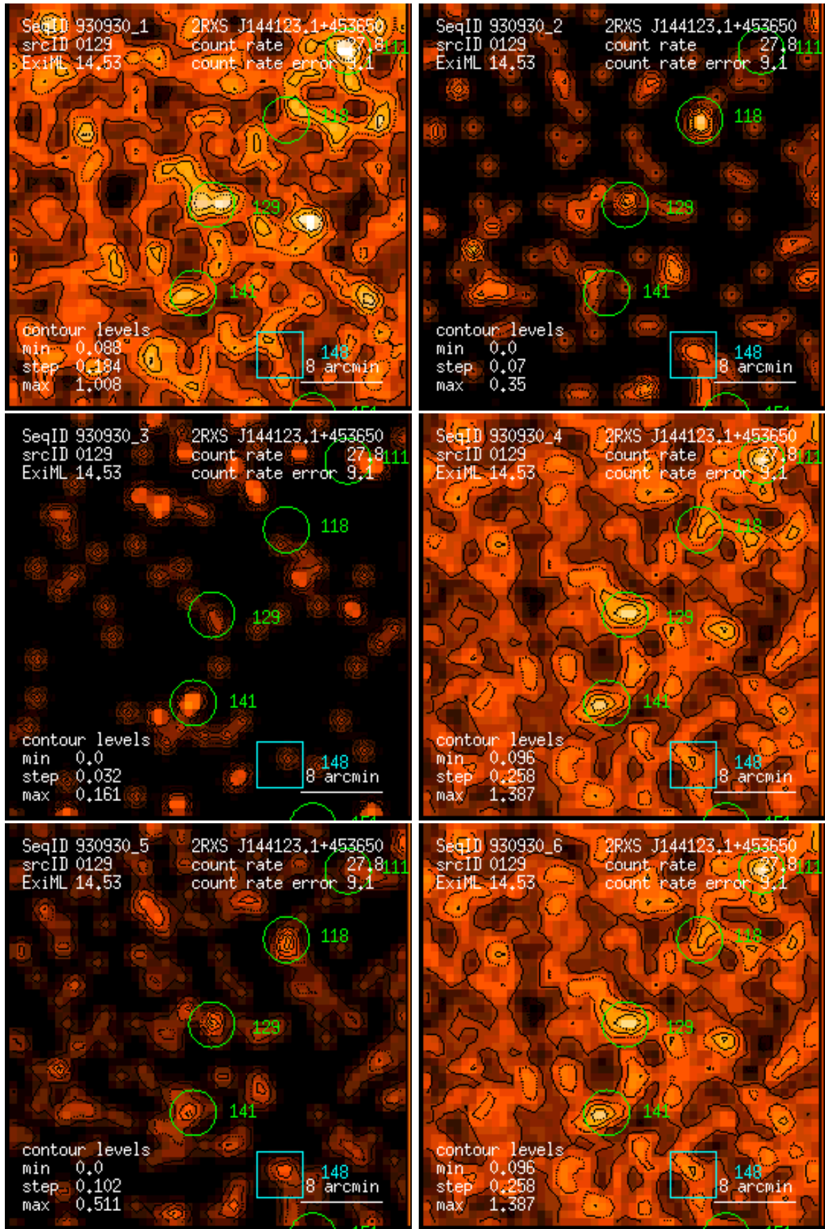
Figure 129: RASS 930930: detection 0129: band rate images, Gaussian filter: (1) PSPC channels 11 – 41, (2) 52 – 90, (3) 91 – 201, (4) 11 – 235, (5) 52 – 201, (6) 11 – 201. Broad band rates in counts/ks. Band rate contour levels in counts/ks/arcmin 2 .
