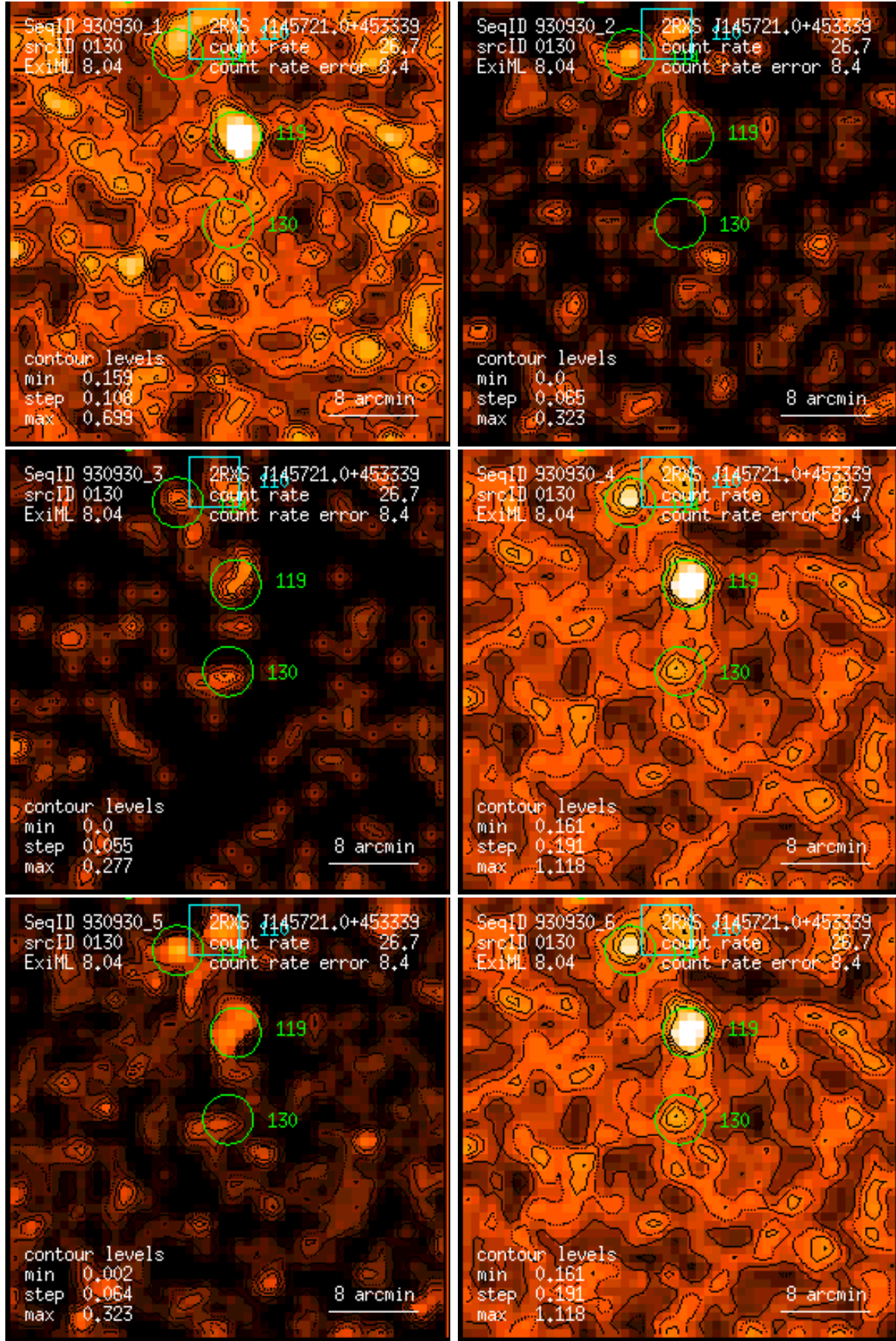
Figure 130: RASS 930930: detection 0130: band rate images, Gaussian filter: (1) PSPC channels 11 – 41, (2) 52 – 90, (3) 91 – 201, (4) 11 – 235, (5) 52 – 201, (6) 11 – 201. Broad band rates in counts/ks. Band rate contour levels in counts/ks/arcmin 2 .
