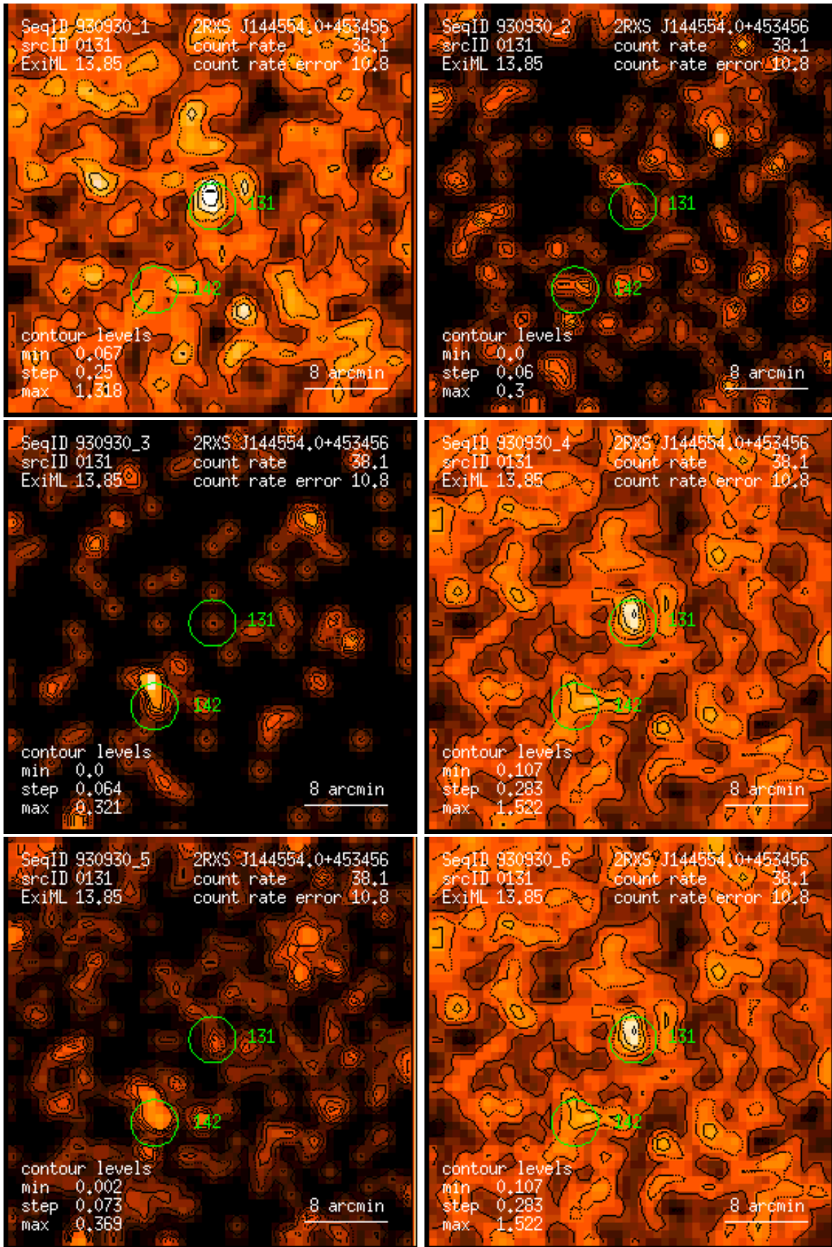
Figure 131: RASS 930930: detection 0131: band rate images, Gaussian filter: (1) PSPC channels 11 – 41, (2) 52 – 90, (3) 91 – 201, (4) 11 – 235, (5) 52 – 201, (6) 11 – 201. Broad band rates in counts/ks. Band rate contour levels in counts/ks/arcmin 2 .
