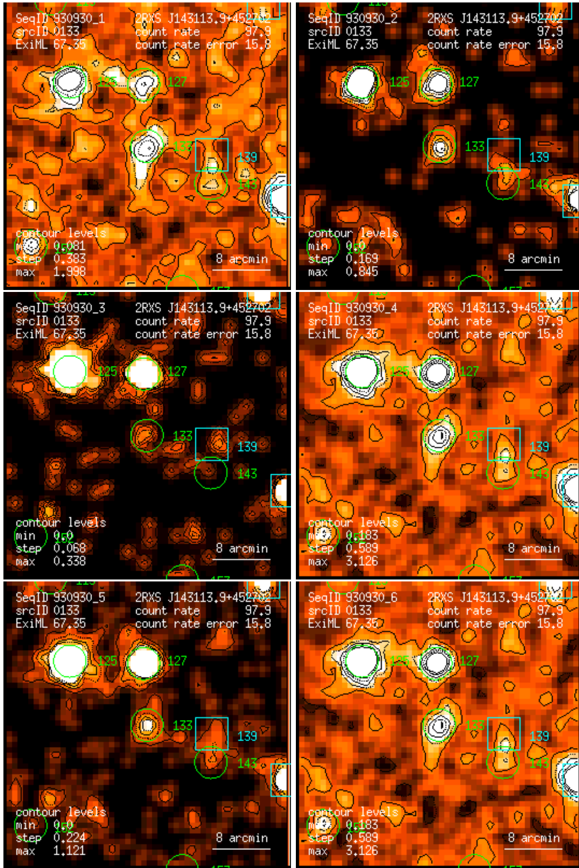
Figure 133: RASS 930930: detection 0133: band rate images, Gaussian filter: (1) PSPC channels 11 – 41, (2) 52 – 90, (3) 91 – 201, (4) 11 – 235, (5) 52 – 201, (6) 11 – 201. Broad band rates in counts/ks. Band rate contour levels in counts/ks/arcmin 2 .
