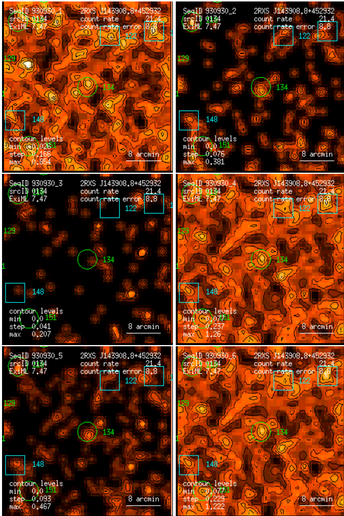
Figure 134: RASS 930930: detection 0134: band rate images, Gaussian filter: (1) PSPC channels 11 – 41, (2) 52 – 90, (3) 91 – 201, (4) 11 – 235, (5) 52 – 201, (6) 11 – 201. Broad band rates in counts/ks. Band rate contour levels in counts/ks/arcmin 2 .
